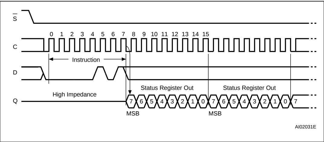
Figure 9. Read Status Register (RDSR) instruction sequence and data-out sequence
