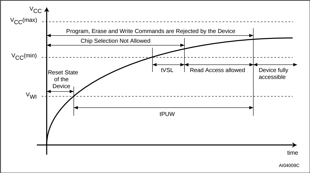
Figure 23. Power-up timing
