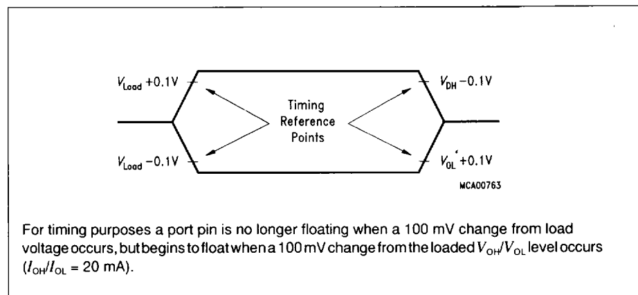
Figure 10 Float Waveforms
