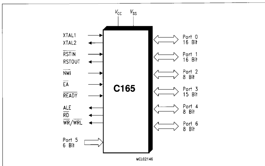
Figure 1 Logic Symbol
