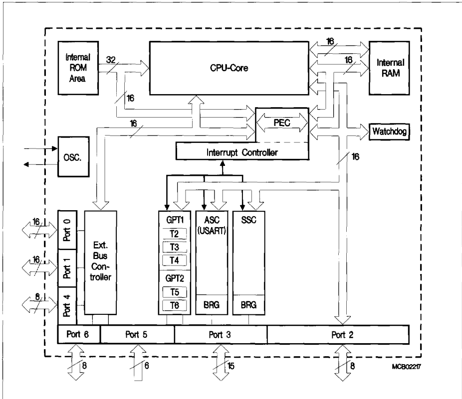
Figure 4 Block Diagram
