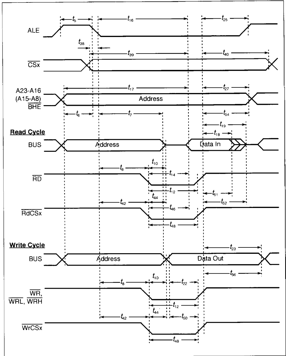
Figure 12-2 External Memory Cycle: Multiplexed Bus, With Read/Write Delay, Extended ALE
