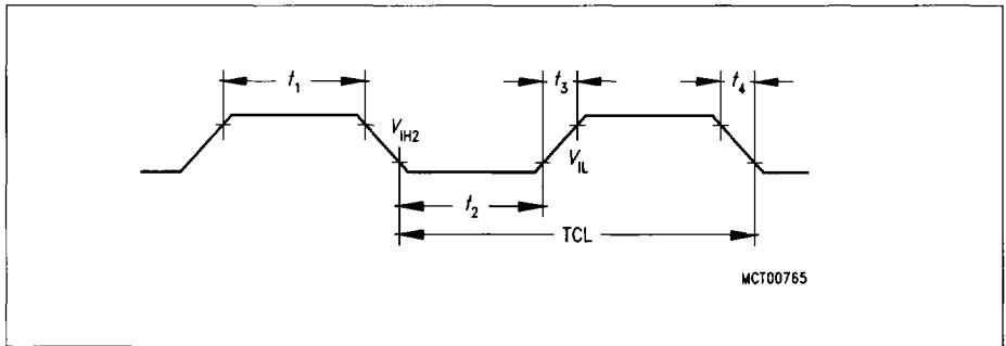
Figure 11 External Clock Drive XTAL1
