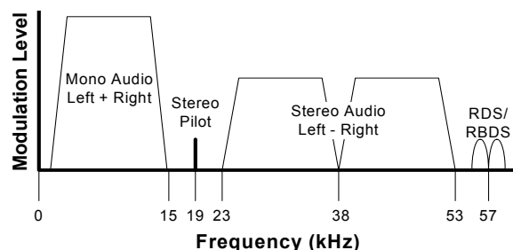
Figure 8. MPX Signal Spectrum
