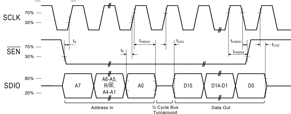
Figure 4. 3-Wire Control Interface Read Timing Parameters
