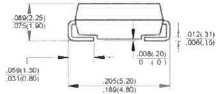
Dimensions in Inches and (millimeters)
