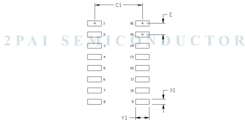
Figure 20.16-Lead Narrow Body SOIC [NB SOIC-16] Land Pattern
