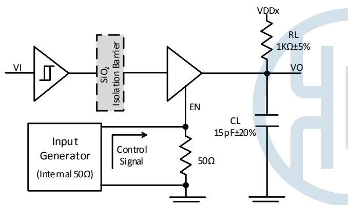
Figure 11. t_{PZL}/t_{PLZ} test circuit
