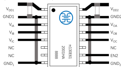
Figure 15. Recommended Printed Circuit Board Layout
