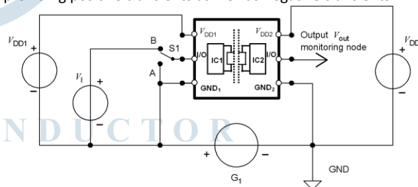
Figure 16. Common-mode transient immunity (CMTI) measurement
