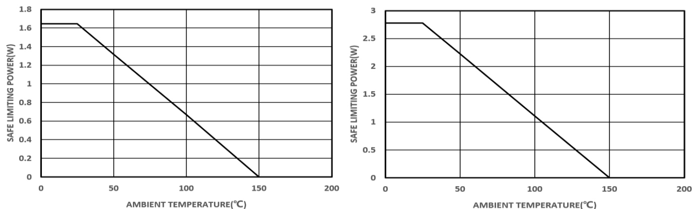
Figure 5. Thermal Derating Curve, Dependence of Safety Limiting Values with Ambient Temperature per VDE (left: \pi 130U3x ; right: \pi 130U6x )
