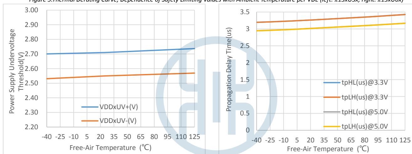
Figure 6. UVLO vs. Free-Air Temperature
