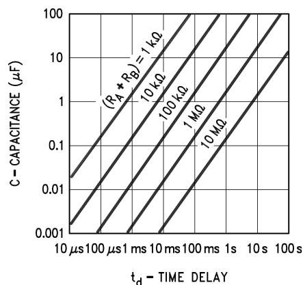
Figure 7-4. Time Delay
