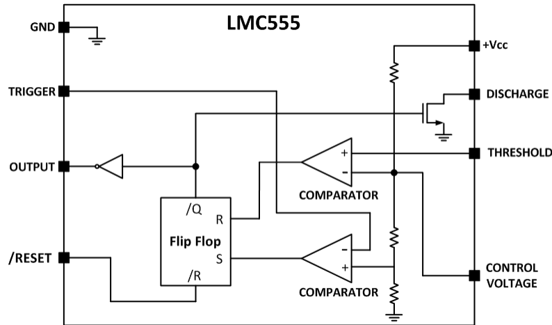
Figure 7-1. Simplified Schematic
