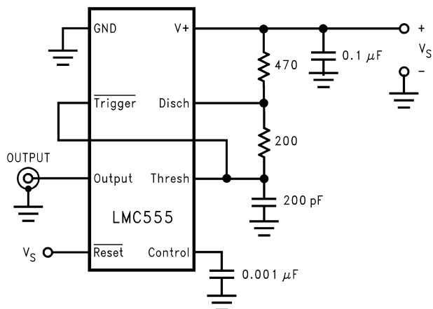
Figure 6-1. Test Circuit
