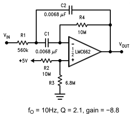
Figure 6-12. 10Hz Band-Pass Filter
