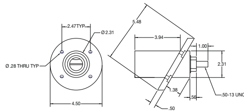
MALE RECEPTACLE 30° ANGLE
