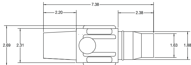
FEMALE CONNECTOR
