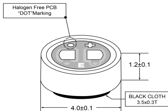
ANGLED VIEW
