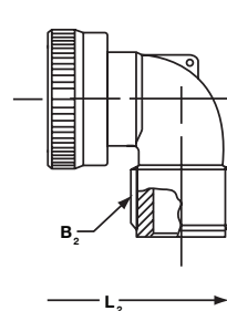
CB6T ENDBELL
