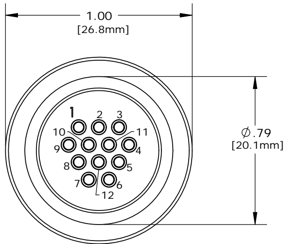
WIRE VIEW W4280-10SG-300 - 10-POS. (11&12 CLOSED) W4280-11SG-300 - 11-POS. (12 CLOSED) W4280-12SG-300 - 12-POS. (ALL OPEN)
