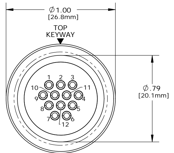
PC TAIL VIEW W4282-10SG-300 - 10-POS. (11&12 CLOSED) W4282-11SG-300 - 11-POS. (12 CLOSED) W4282-12SG-300 - 12-POS. (ALL OPEN)
