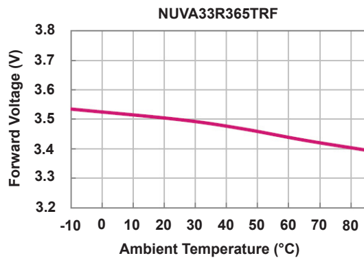
AMBIENT TEMPERATURE VS. FORWARD VOLTAGE @ 500mA If
