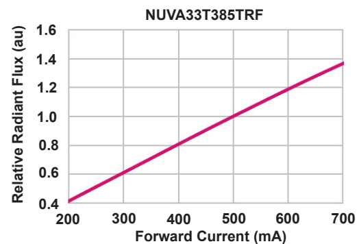
FORWARD CURRENT VS. RELATIVE RADIANT FLUX @ +25°C
