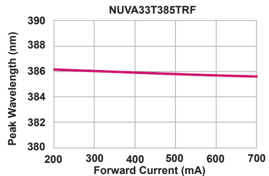
FORWARD CURRENT VS. PEAK WAVELENGTH @ +25°C
