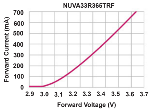
FORWARD VOLTAGE VS. FORWARD CURRENT @ +25°C
