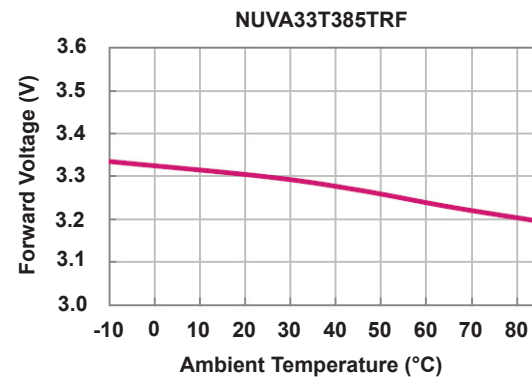
AMBIENT TEMPERATURE VS. FORWARD VOLTAGE @ 500mA If
