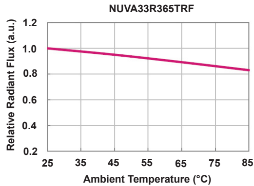
AMBIENT TEMPERATURE VS. RELATIVE RADIANT FLUX @ 500mA If
