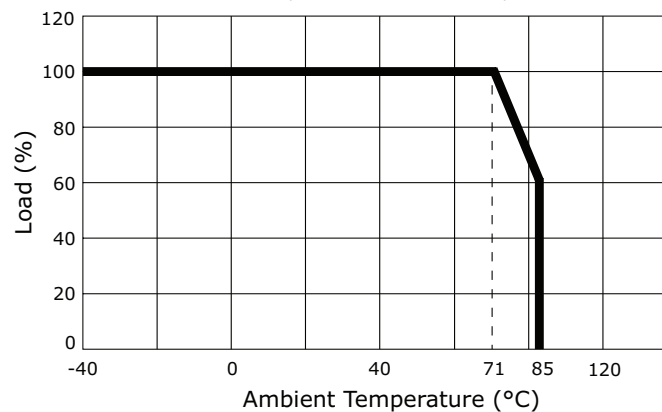
Temperature Derating Curve (Natural Convention)
