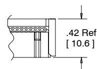
Assembled Height Without Strain Relief
