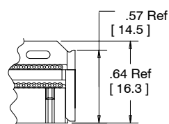
Assembled Height with Standard Plastic Strain Relief
