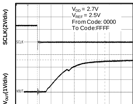
Full-Scale Settling Time(2.7V Rising Edge)
