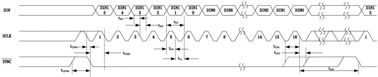
Figure 2. 16-Bit Serial-Interface Timing Diagram (TPC114S1)
