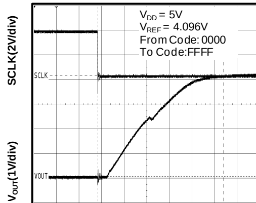
Full-Scale Settling Time(5V Rising Edge)
