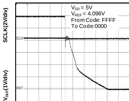
Full-Scale Settling Time(5V Falling Edge)
