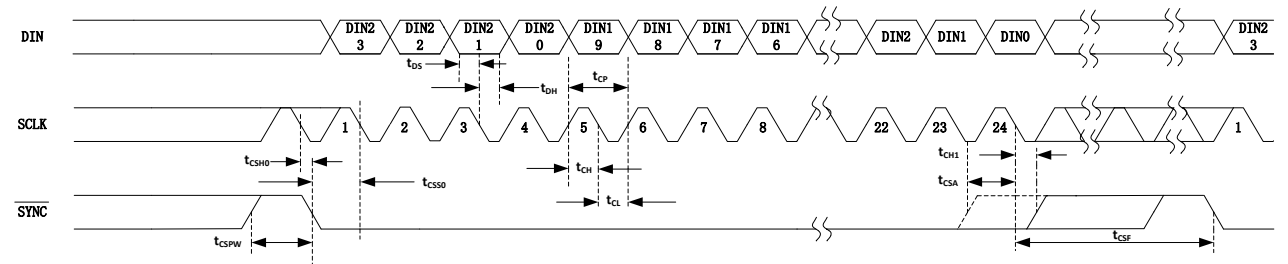
Figure 3. 24-Bit Serial-Interface Timing Diagram (TPC116S1)
