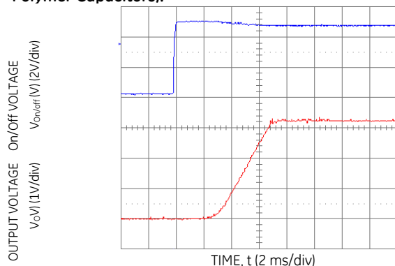
Figure 14. Typical Start-Up Using Remote On/Off ( V_{in} = 5.0\text{ Vdc} , V_o = 3.3\text{ Vdc} , I_o = 16.0\text{ A} ).
