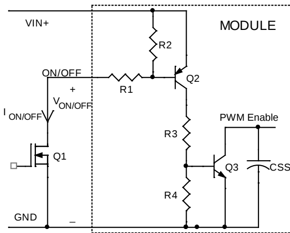
Figure 28. Remote On/Off Implementation.
