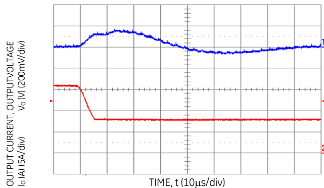
Figure 13. Transient Response to Dynamic Load Change from 100% of 50% full load ( V_o = 5.0\text{ Vdc} , C_{ext} = 2 \times 150\text{ }\mu\text{F} Polymer Capacitors).
