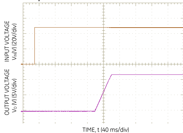
Figure 4. Typical Start-Up Using Vin with Remote On/Off enabled, negative logic version shown.
