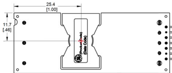
Figure 25. Pick and Place Location.
