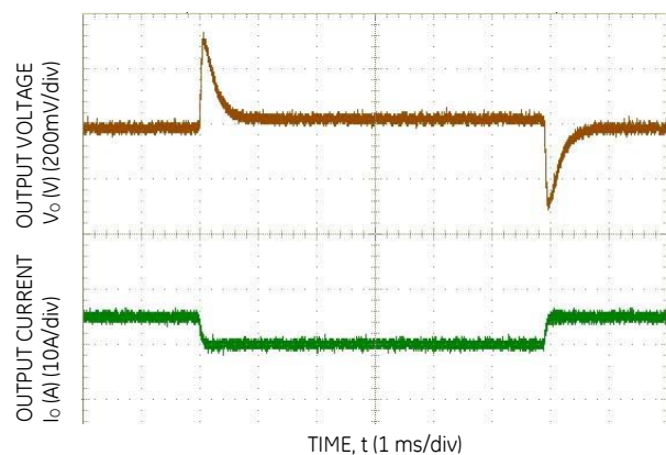
Figure 12. Typical Transient Response to Step Change in Load from 50% to 75% to 50% of Full Load at 48Vdc Input and C_0 = 220\mu F Polymer, with -02 option.
