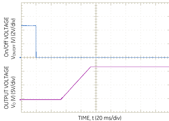
Figure 3. Typical Start-Up Using Remote On/Off with Vin applied, negative logic version shown.
