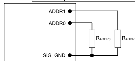
Figure 28. Circuit showing connection of resistors used to set the PMBus address of the module.
