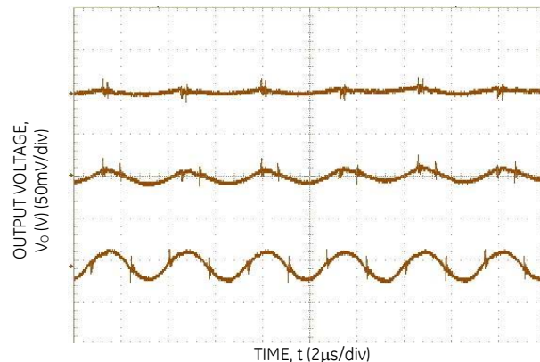
Figure 10. Typical Output Ripple and Noise at Room Temperature I_o = I_{o,max} and C_{0min} .
