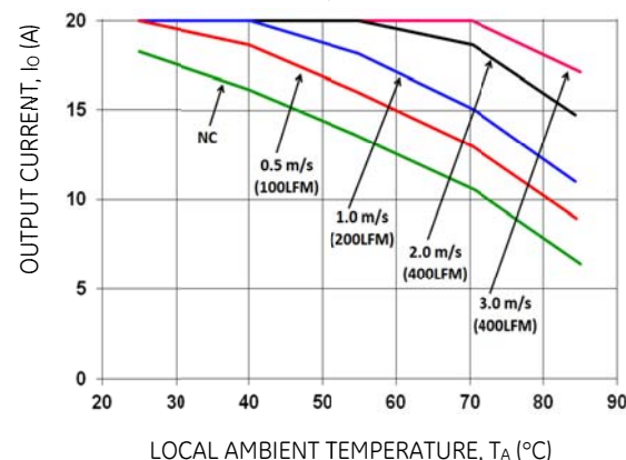
Figure 22. Output Current Derating for the Base Plate EBDW020A0Bxx-H in the Transverse Orientation; Airflow Direction from V_{in}(-) to V_{in}(+) ; V_{in} = 48\text{V} .
