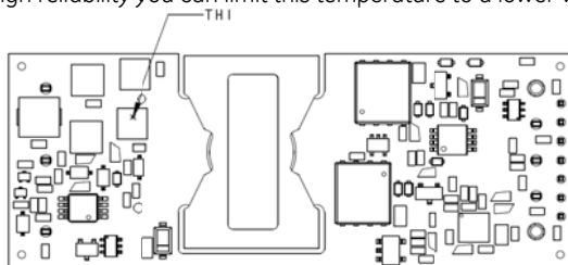
Figure 19. Location of the thermal reference temperature TH_1 . Do not exceed 113^\circ\text{C} .
