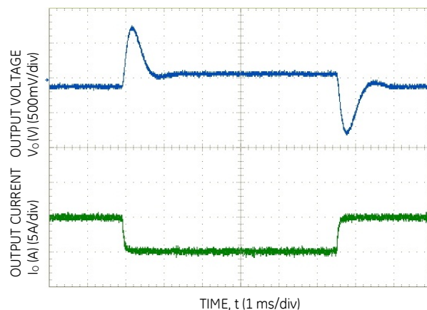
Figure 5. Typical Transient Response to Step Change in Load from 25% to 50% to 25% of Full Load at 48Vdc Input and C_o = 470\mu\text{F} Polymer, without -02 option.
