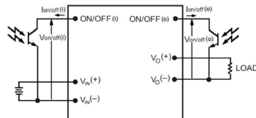
Figure 16. Remote On/Off Implementation.
