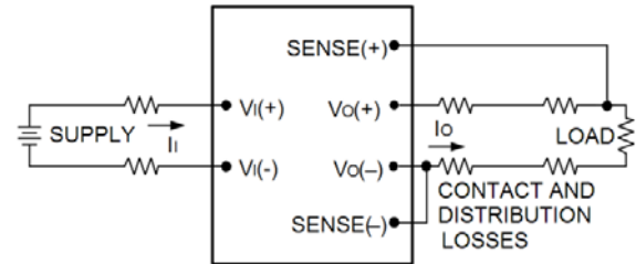
Figure 17. Circuit Configuration for remote sense.
