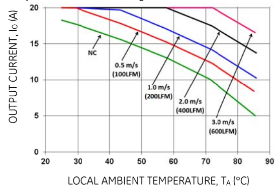
Figure 21. Output Current Derating for the Open Frame EBDW020A0B in the Transverse Orientation; Airflow Direction from V_{in}(-) to V_{in}(+) ; V_{in} = 48\text{V} .
