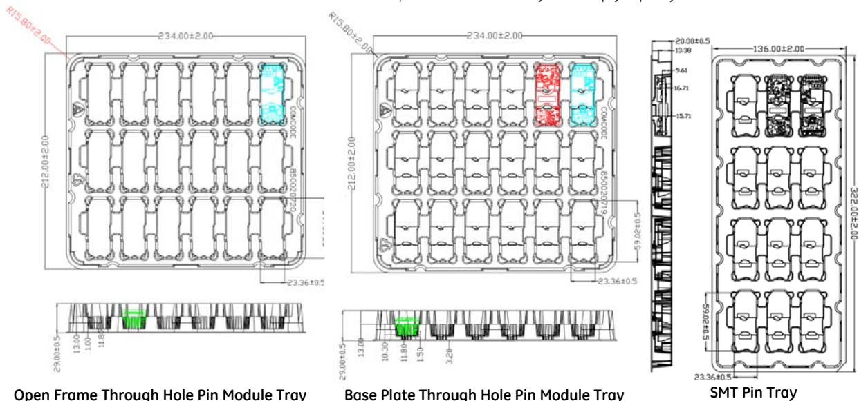
Open Frame Through Hole Pin Module Tray Figure 27. EBDW020 Packaging Tray
