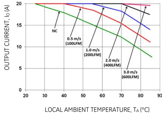
Figure 23. Output Current Derating for the Base Plate EBDW020A0Bxx-H and 0.25" heat sink in the Transverse Orientation; Airflow Direction from Vin(-) to Vin(+); Vin = 48V.
