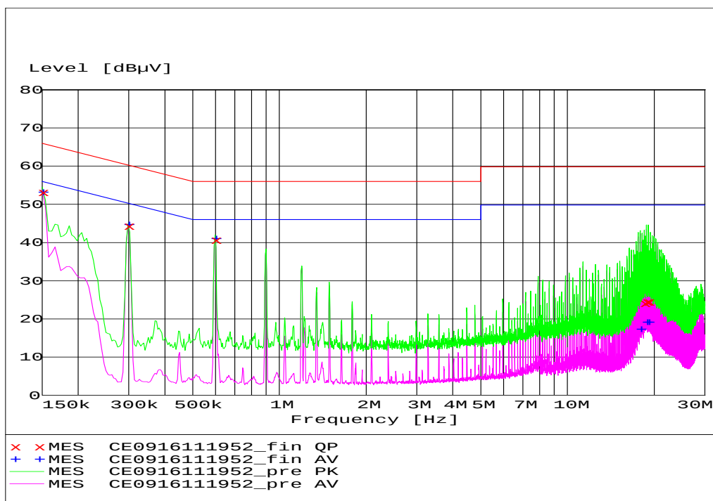
Figure 26. EMC Considerations.
