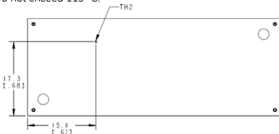
Figure 20. Location of the thermal reference temperature TH_2 for Baseplate module. Do not exceed 110^\circ\text{C} .
