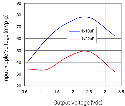
Figure 40. Input ripple voltage for various output voltages with 1x10 µF or 1x22 µF ceramic capacitors at the input (2A load). Input voltage is 5V. Scope BW: 20MHz.
