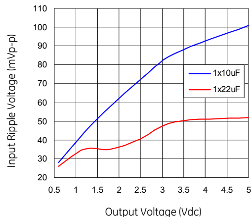
Figure 41. Input ripple voltage for various output voltages with 1x10 µF or 1x22 µF ceramic capacitors at the input (2A load). Input voltage is 12V. Scope BW: 20MHz
