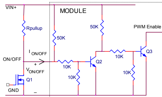
Figure 43. Circuit configuration for using positive On/Off logic.
