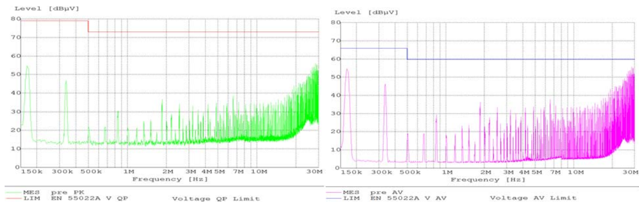
Figure 23. EMC Filter
