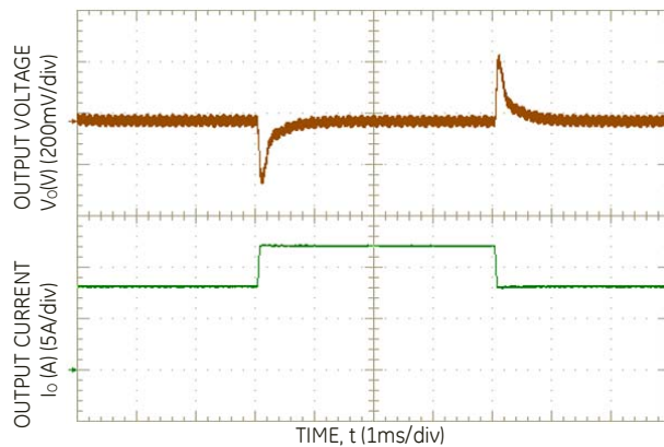
Figure 3. Dynamic Load Change Transient Response from 50% to 75% to 50% of Full Load at Room Temperature and 48 Vin; 0.1A/µS, C_{o,ext} = 470\mu F .
