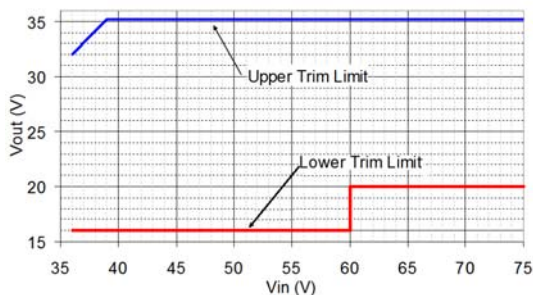
Figure 12. Output Voltage Trim Limits vs. Input Voltage.
