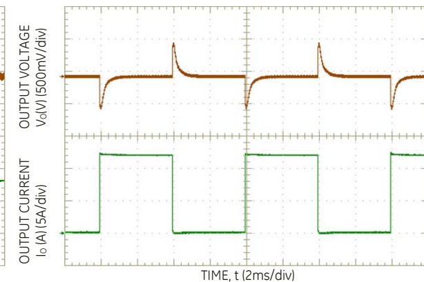
Figure 6. Dynamic Load Change Transient Response from 0 % to 75% to 0% of Full Load at Room Temperature and 48 Vin; 2.0A/µS, C_{o,ext} = 880\mu F .
