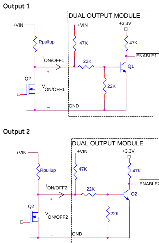
Figure 39. Circuit configuration for using positive On/Off logic.
