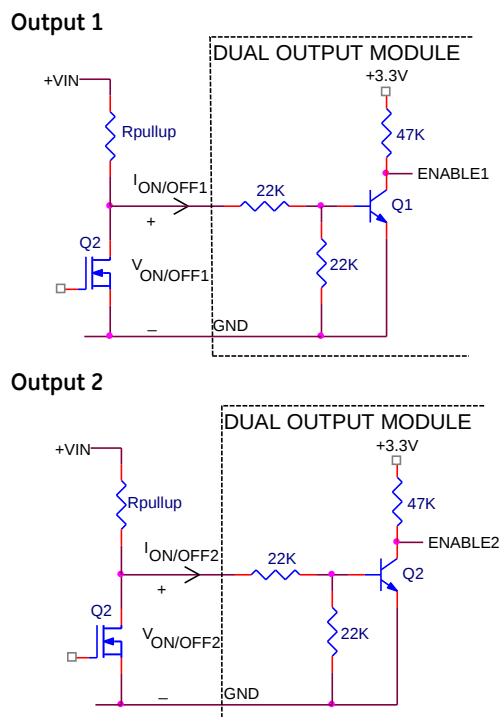
Figure 40. Circuit configuration for using negative On/Off logic.
