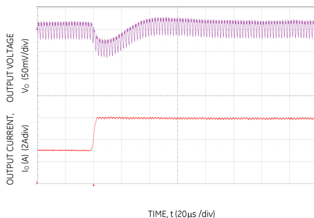
Figure 22. Transient Response to Dynamic Load Change on one output from 50% to 100% at 12V in , C_{out} = 2 \times 47\mu\text{F} + 1 \times 330\mu\text{F} , C_{Tune} = 1500\text{pF} & R_{Tune} = 300\Omega
