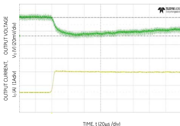
Figure 16. Transient Response to Dynamic Load Change from 50% to 100% at 12Vin, C_{out}=4 \times 47\mu\text{F} + 1 \times 330\mu\text{F} , C_{Tune}=15\text{nF} , R_{Tune}=300
