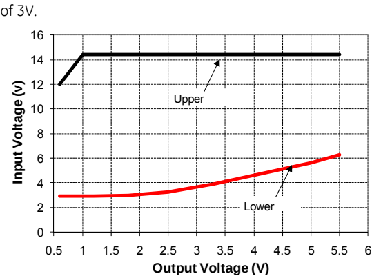
Figure 40. Output Voltage vs. Input Voltage Set Point Area plot showing limits where the output voltage can be set for different input voltages.
