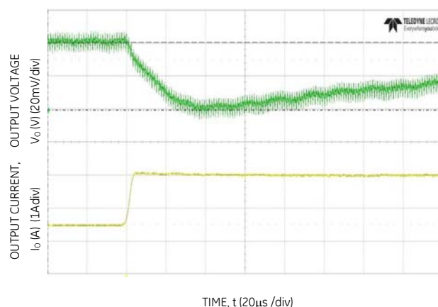
Figure 22. Transient Response to Dynamic Load Change from 50% to 100% at 12Vin, C_{out}=4 \times 47 \mu\text{F} + 1 \times 330 \mu\text{F} , C_{Tune}=10\text{nF} , R_{Tune}=300 \Omega
