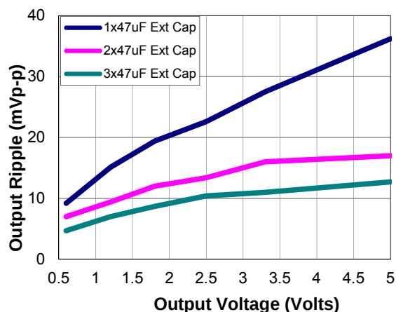
Figure 38. Output ripple voltage with external 1x47 \mu F, 2x47 \mu F, or 3x47 \mu F ceramic capacitors at the output (3A load). Input voltage is 12V. Scope BW Limited to 20MHz.
