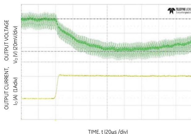
Figure 28. Transient Response to Dynamic Load Change from 50% to 100% at 12Vin, C_{out}=2 \times 47\mu\text{F} + 1 \times 330\mu\text{F} , C_{Tune}=6800\text{pF} , R_{Tune}=300
