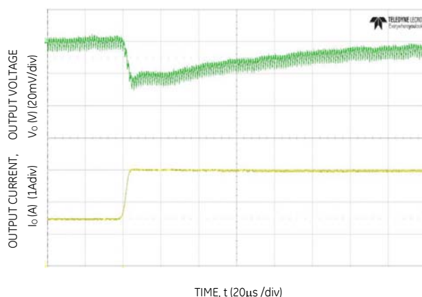
Figure 34. Transient Response to Dynamic Load Change from 50% to 100% at 12Vin, C_{out}=2 \times 47 \mu F + 1 \times 330 \mu F , C_{Tune}=2700pF , R_{Tune}=300\Omega
