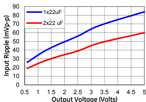
Figure 37. Input ripple voltage for various output voltages with 1x22 \mu F or 2x22 \mu F ceramic capacitors at the input (3A load). Input voltage is 12V. Scope BW Limited to 20MHz
