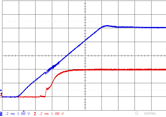
Figure 33. Input/Output Start-Up Characteristics : 5.0VIN,2.0VOUT,1ms input ramp.
