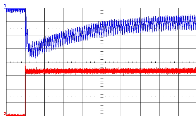
Blue(upper)=Vout 20mV/div Red(lower)=Vin1A/div 10μs/div
