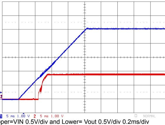
Figure 34. Input/Output Start-Up Characteristics : 5.0VIN,2.0VOUT,20ms input ramp.
