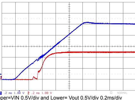
Figure 35. Input/Output Start-Up Characteristics : 5.0VIN,2.5VOUT,1ms input ramp.
