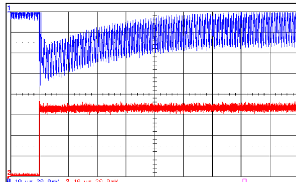
Blue(upper)=Vout 20mV/div Red(lower)=1A/div 10μs/div
