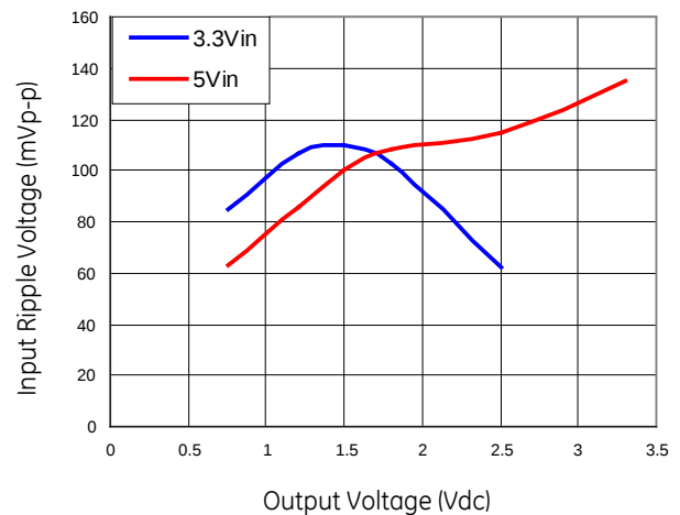
Figure 28. Input ripple voltage for various outputs with 1x22 μF ceramic capacitor at the input (full-load).
