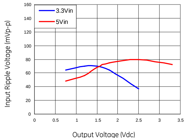
Figure 29. Input ripple voltage for various outputs with 1x47 μF ceramic capacitor at the input (full load).
