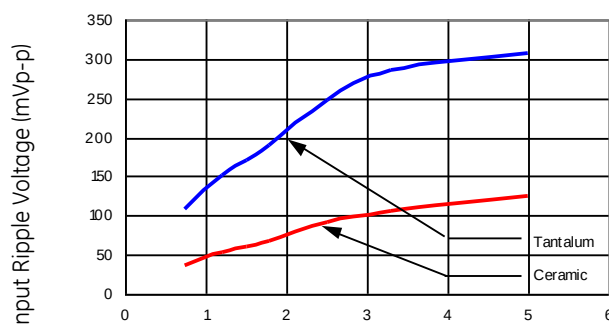
Figure 27. Input ripple voltage for various output with 2x47 µF tantalum capacitors and with 2x22 µF ceramic capacitors at the input (80% of I_{O,max} ).
