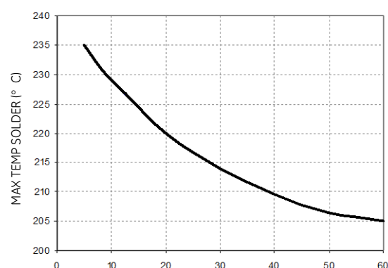
Figure 36. Time Limit Curve Above 205°C for Tin/Lead (Sn/Pb) process.
