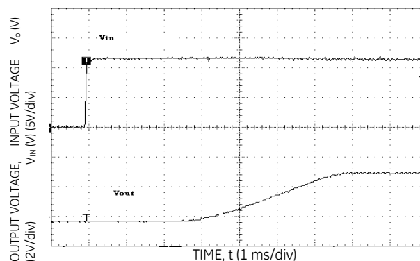
Figure 16. Typical Start-Up with application of V_{in} with ( V_{in} = 12 Vdc, V_o = 3.3 Vdc, I_o = 6 A).
