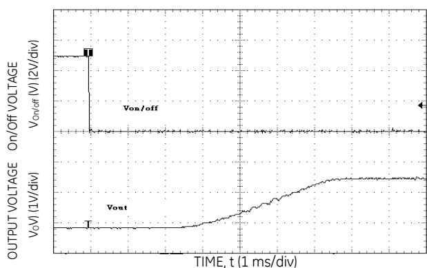
Figure 15. Typical Start-Up Using Remote On/Off with Low-ESR external capacitors (7x150 \mu F Polymer)
