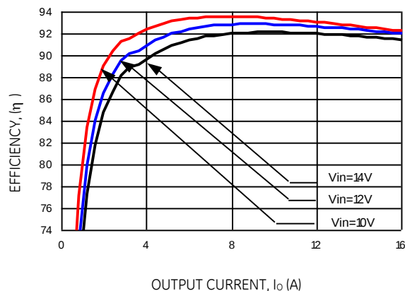
Figure 5. Converter Efficiency versus Output Current ( V_{out} = 3.3Vdc ).
