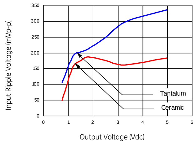
Figure 26. Input ripple voltage for various output with 6x47 μF tantalum capacitors and with 6x22 μF ceramic capacitors at the input (full load).
