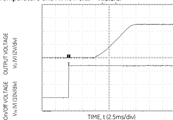
Figure 11. Typical Start-up Using Remote On/Off ( V_{IN} = 24V , I_o = I_{o,max} ).
