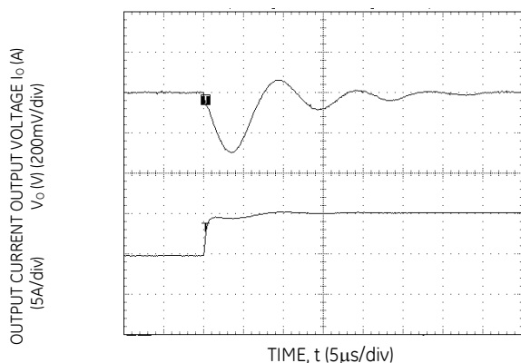
Figure 9. Transient Response to Dynamic Load change from 50% to 100% of full load with di/dt of 5A/μs.
