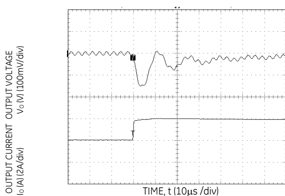
Figure 15. Transient Response to Dynamic Load change from 50% to 100% of full load with di/dt of 5A/μs.
