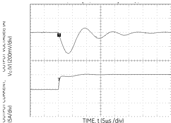
Figure 3. Transient Response to Dynamic Load Change from 50% to 100% of full load with di/dt of 5A/μs.
