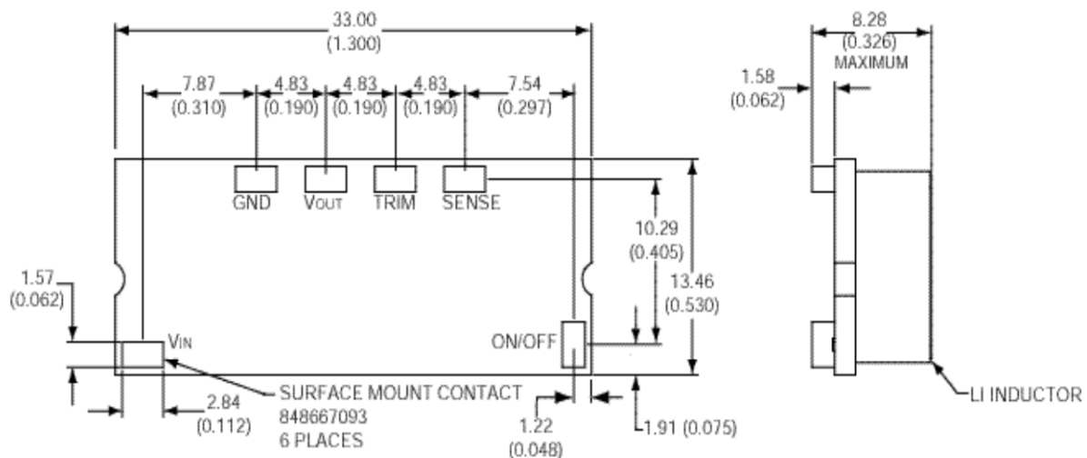
BOTTOM VIEW OF BOARD
