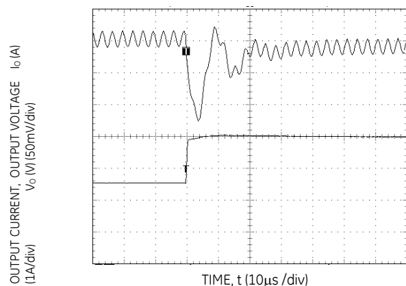
Figure 21. Transient Response to Dynamic Load change from 50% to 100% of full load with di/dt of 5A/μs.
