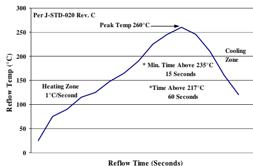
Figure 46. Recommended linear reflow profile using Sn/Ag/Cu solder.
