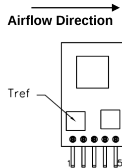
Figure 54. T_{ref} Temperature measurement location.
