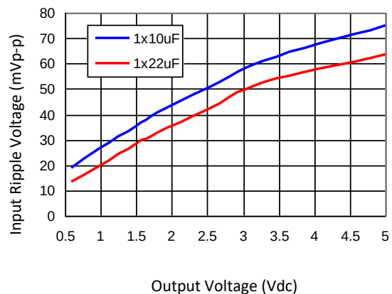
Figure 46. Input ripple voltage for various output voltages with 1x10 μF or 1x22 μF ceramic capacitors at the input (3A load). Input voltage is 12V.
