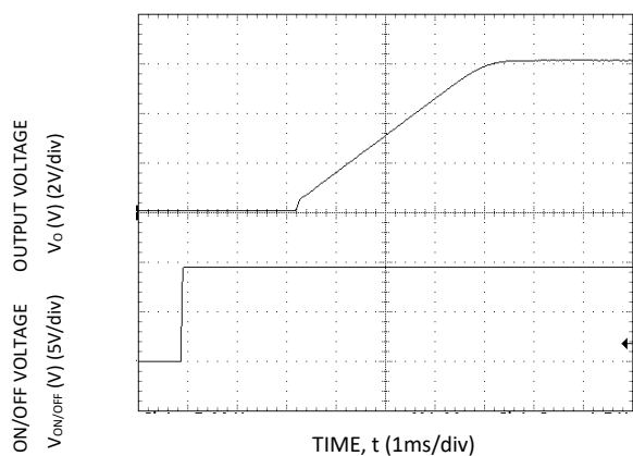
Figure 41. Typical Start-up Using On/Off Voltage ( I_o = I_{o,max} ).
