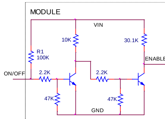
Figure 48. Remote On/Off Implementation. Resistor R1 is absent in the -49Z option module.
