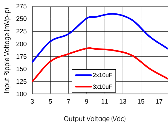
Figure 29. Input ripple voltage for various output voltages with 2 \times 10 \mu F or 3 \times 10 \mu F ceramic capacitors at the input (maximum load). Input voltage is 28V.
