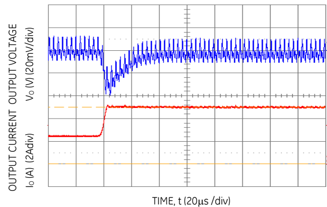
Figure 4. Transient Response to Dynamic Load Change from 50% to 100% at 28V in , C ext = 10μF ceramic + 330μF polymer, C Tune =10nF & R Tune =150Ω
