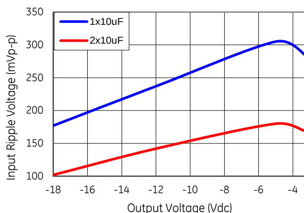
Figure 63. Input ripple voltage with 1x10 \mu F or 2x10 \mu F ceramic capacitors at the input (max load).
