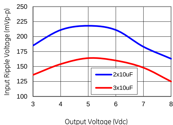
Figure 28. Input ripple voltage for various output voltages with 2 \times 10 \mu F or 3 \times 10 \mu F ceramic capacitors at the input (maximum load). Input voltage is 12V.
