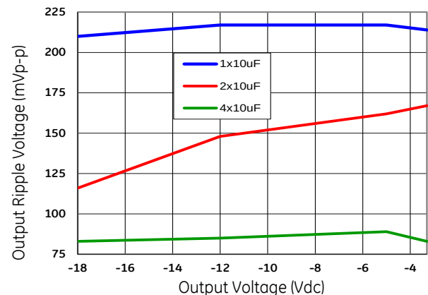
Figure 68. Output ripple with 1x10μF, 2x10μF or 4x10μF output ceramic capacitors (max load).
