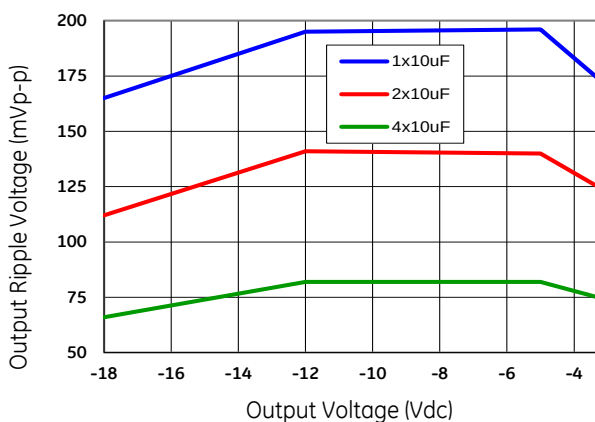
Figure 66. Output ripple with 1x10μF, 2x10μF or 4x10μF output ceramic capacitors (max load).
