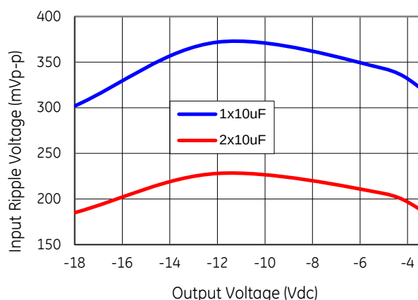
Figure 65. Input ripple voltage with 1x10 \mu F or 2x10 \mu F input ceramic capacitors (max load).
