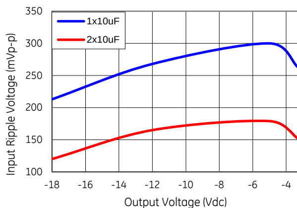
Figure 64. Input ripple voltage with 1x10 \mu F or 2x10 \mu F ceramic capacitors at the input (max load).
