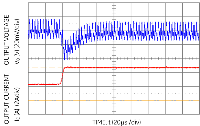
Figure 10. Transient Response to Dynamic Load Change from 50% to 100% at 28Vin, C_{ext} = 10\mu F ceramic + 330 \mu F polymer, C_{Tune}=10nF & R_{Tune}=150\Omega
