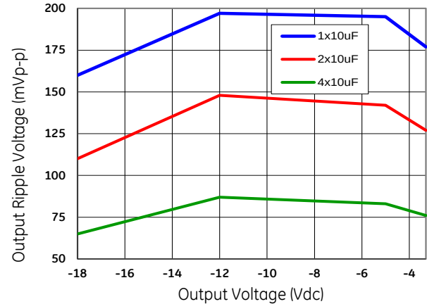
Figure 67. Output ripple with 1x10μF, 2x10μF or 4x10μF output ceramic capacitors (max load).
