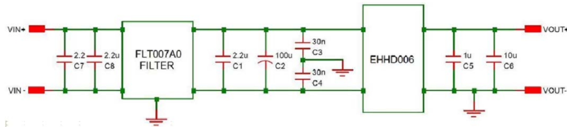
Figure 25. EMC Considerations
