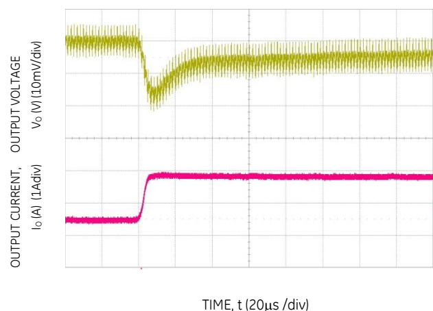
Figure 10. Transient Response to Dynamic Load Change from 50% to 100% at 12V IN , C out = 1x47μF+1x330μF, C Tune =10nF & R Tune =267
