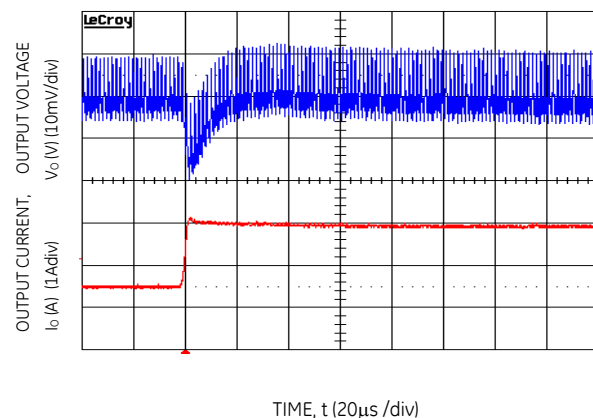
Figure 16. Transient Response to Dynamic Load Change from 50% to 100% at 12V in , C out -1x47μF+1x330μF, C Tune -10nF & R Tune -261
