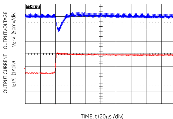
Figure 28. Transient Response to Dynamic Load Change from 50% to 100% at 12Vin, C_{out}=2\times 47\mu\text{F} , C_{Tune}=2200\text{pF} & R_{Tune}=261
