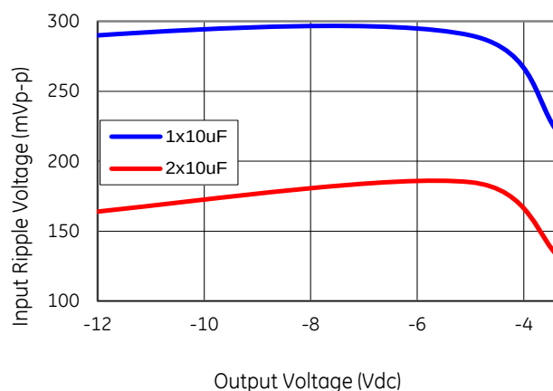
Figure 61. Input ripple voltage with 1x10 \mu F or 2x10 \mu F input ceramic capacitors (max load).
