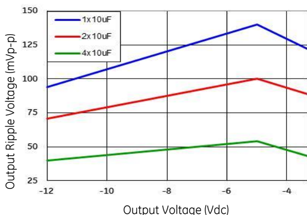
Figure 62. Output ripple with 1x10μF, 2x10μF & 4x10μF output ceramic capacitors (max load).
