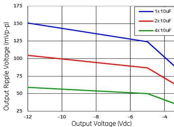
Figure 64. Output ripple with 1x10μF, 2x10μF & 4x10μF output ceramic capacitors (max load).
