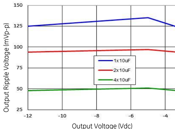
Figure 63. Output ripple with 1x10μF, 2x10μF & 4x10μF output ceramic capacitors (max load).
