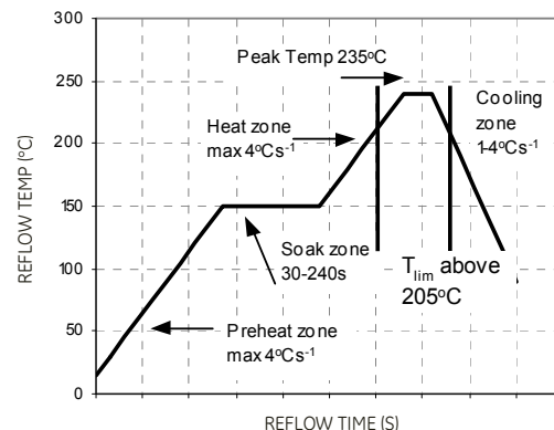
Figure 26. Reflow Profile for Tin/Lead (Sn/Pb) process.
