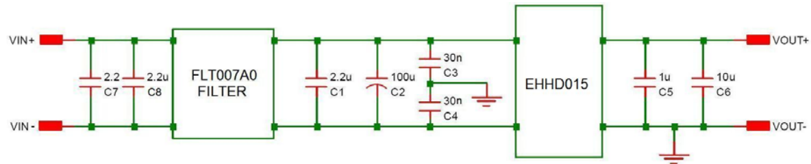
Figure 29. EMC Considerations
