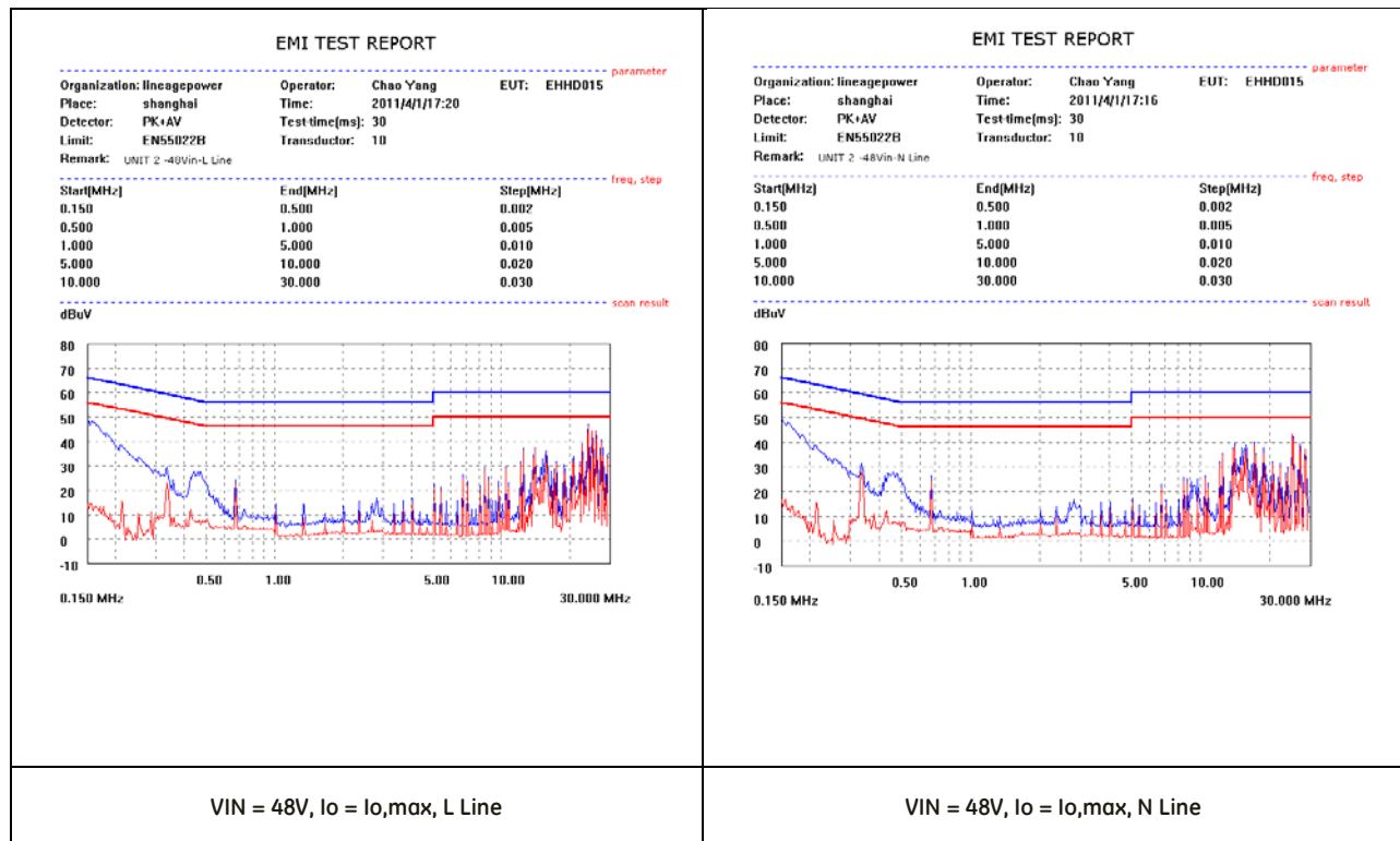
Figure 29. EMC Considerations
