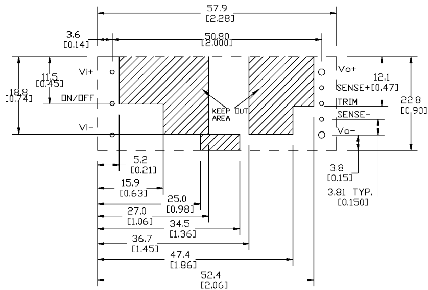
TH Recommended Pad Layout (Component Side View)
