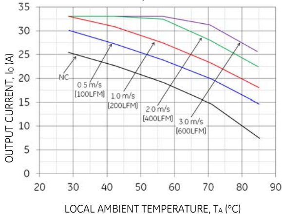
Figure 20. Output Current Derating for the Base plate QBDW033A0B-H in the Transverse Orientation; Airflow Direction from Vin(-) to Vin(+); Vin = 48V.
