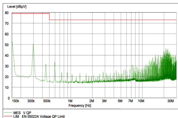
Figure 26. EMC Considerations
