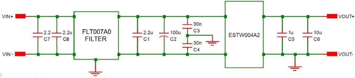
Figure 23. EMC Considerations
