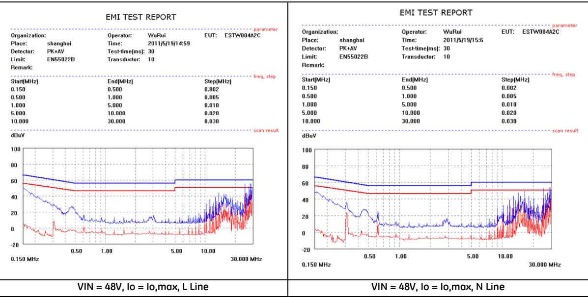
Figure 23. EMC Considerations
