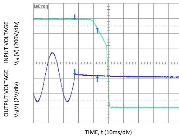
Figure 8. Typical Hold-up waveforms ( V_{IN} = 230V , 100% load).
