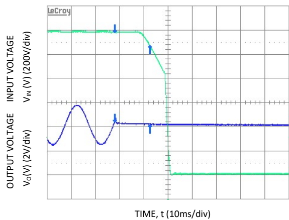
Figure 7. Typical Hold-up waveforms ( V_{IN} = 115V , 100% load).
