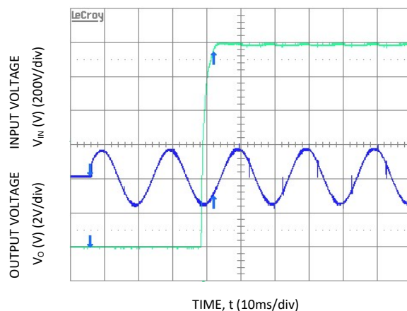
Figure 5. Typical Start-up ( V_{IN} = 115\text{Vac} ).
