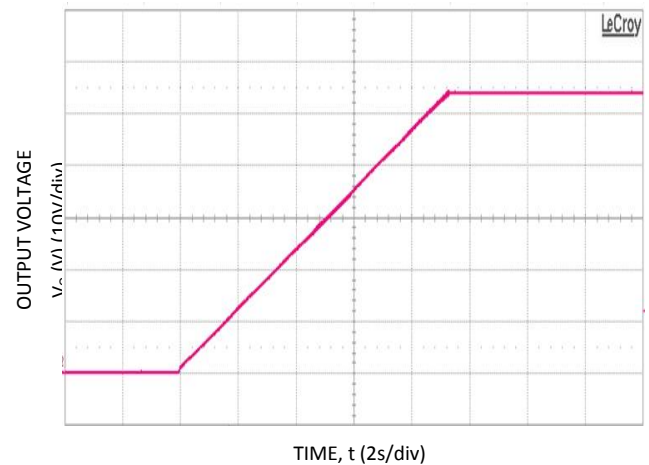
Figure 10. 54V DC soft start, full load, V IN = 230V AC - RS485 mode with 4700μF external capacitance.
