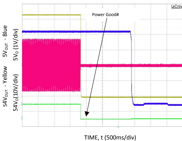
Figure 15. Turn-OFF at full load, V_{IN}=230V_{AC}
