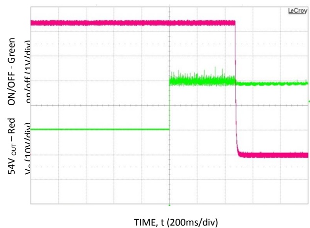
Figure 16. 54V DC turn-OFF delay when ON/OFF is di-asserted, V_{IN}=230V_{AC} - I 2 C mode.
