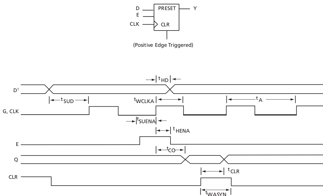
Figure 1-14 • Flip-Flops and Latches (RT1425A, A1425A, RT1460A, A1460A, RT14100A, A14100A)
