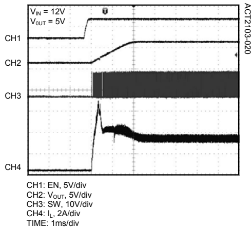
Start Up with EN (Load 3A)
