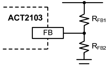
Output Voltage Setting
