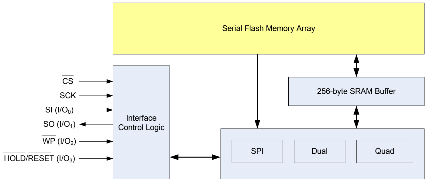
Figure 3-1. Block Diagram
