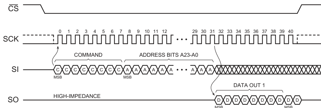
Figure 5-6. SPI Transfer — Command, Address, and Data — Read Operation with No Dummy Bytes
