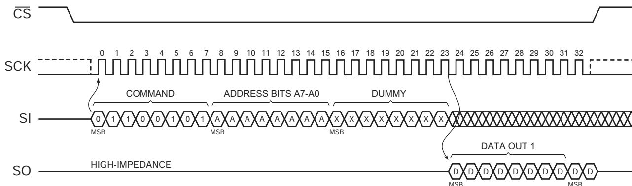
Figure 7-2. Status Register Read Operation Showing 8-bit Address Field
