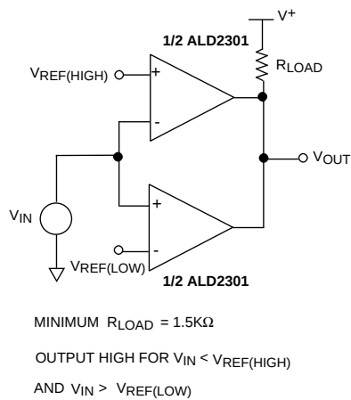
DUAL LIMIT WINDOW COMPARATOR
