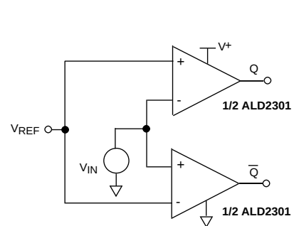
VOLTAGE COMPARATOR WITH COMPLEMENTARY OUTPUTS
