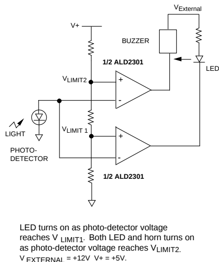
DUAL LIMIT PHOTO-DETECTOR MONITOR
