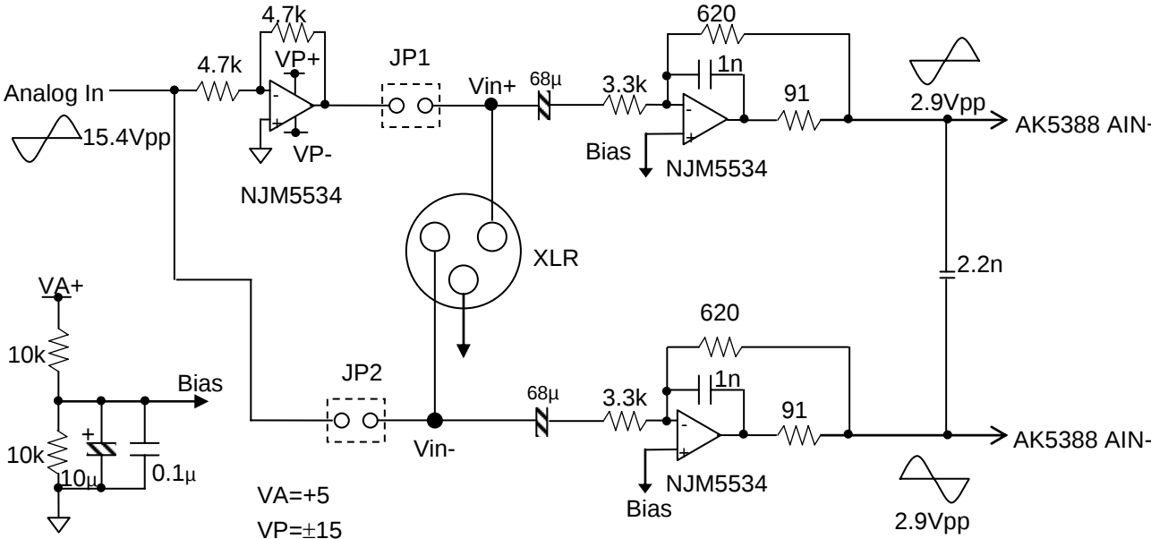
Figure 23. Input Buffer example1
