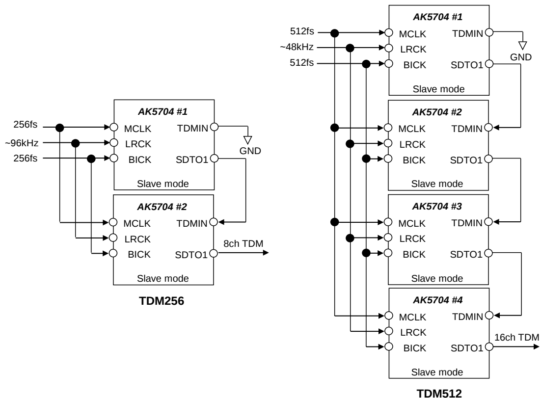
Figure 28. Cascade Connection
