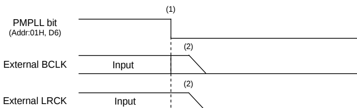
Figure 66. Clock Stopping Sequence (2)
