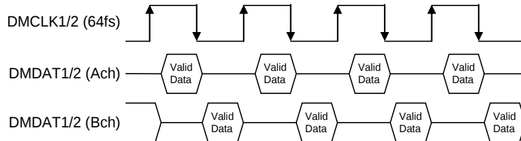
Figure 36. Digital MIC Data Input/Output Timing (DCLKP1/2 bit = "1")
