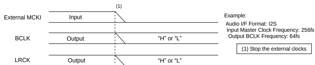
Figure 69. Clock Stopping Sequence (5)
