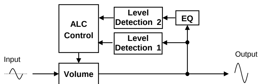
Figure 39. ALC Block
