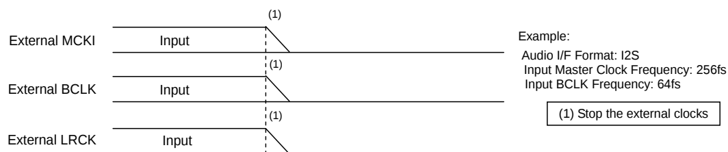
Figure 68. Clock Stopping Sequence (4)
