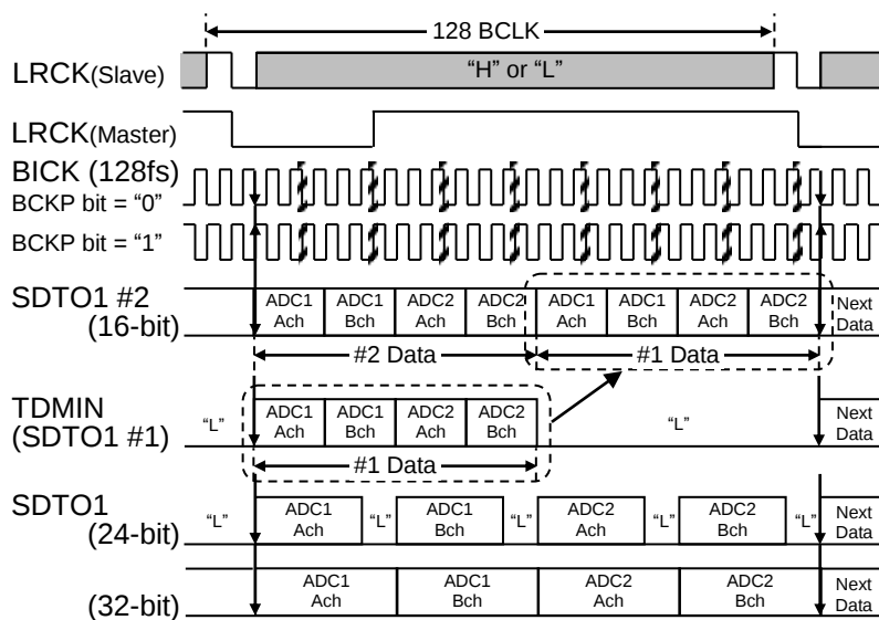
Figure 22. Mode 8/12 Timing (TDM128 mode, I²S Compatible)
