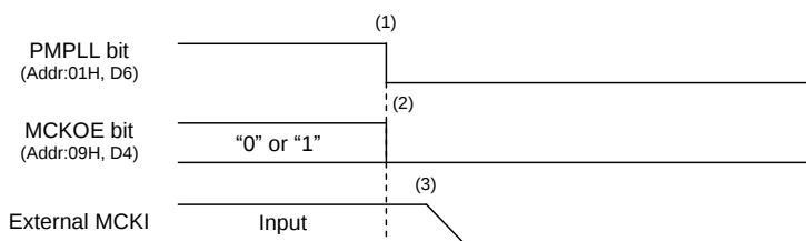
Figure 65. Clock Stopping Sequence (1)
