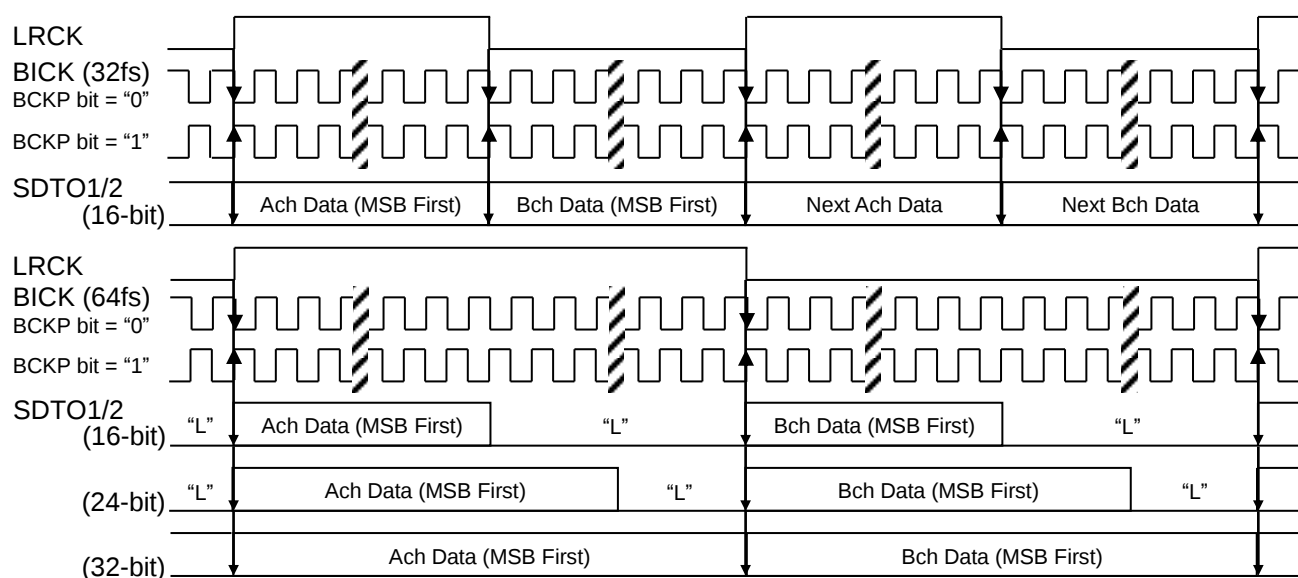
Figure 19. Mode 1/5 Timing (Normal mode, MSB Justified)
