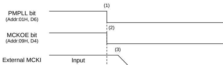
Figure 67. Clock Stopping Sequence (3)
