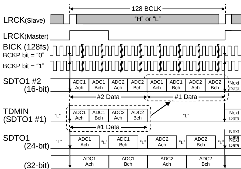
Figure 23. Mode 9/13 Timing (TDM128 mode, MSB Justified)
