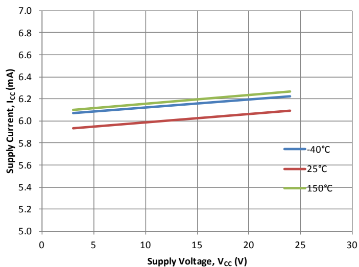
Average Supply Current (Low) vs. Supply Voltage
