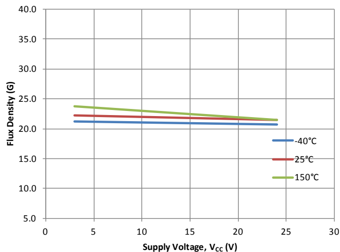
Average B_{RP} vs. Supply Voltage
