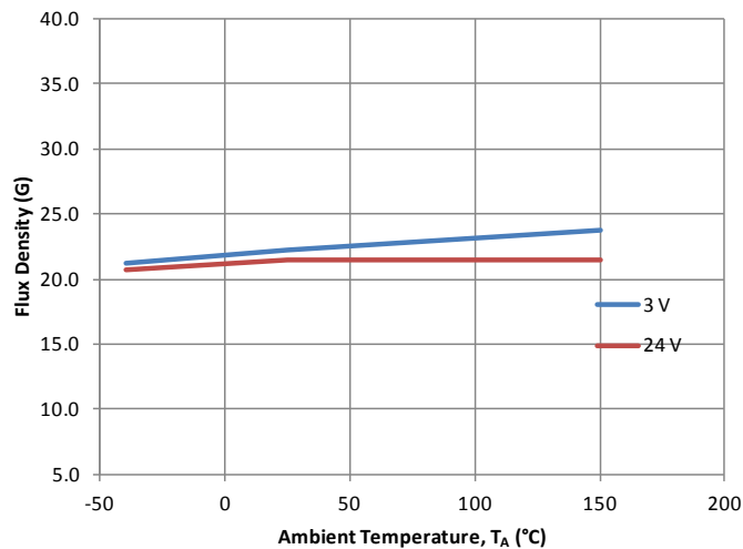
Average B_{RP} vs. Temperature
