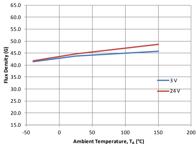
Average B_{HYS} vs. Temperature
