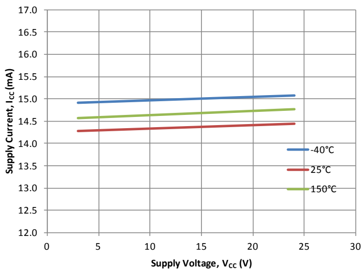
Average Supply Current (High) vs. Supply Voltage
