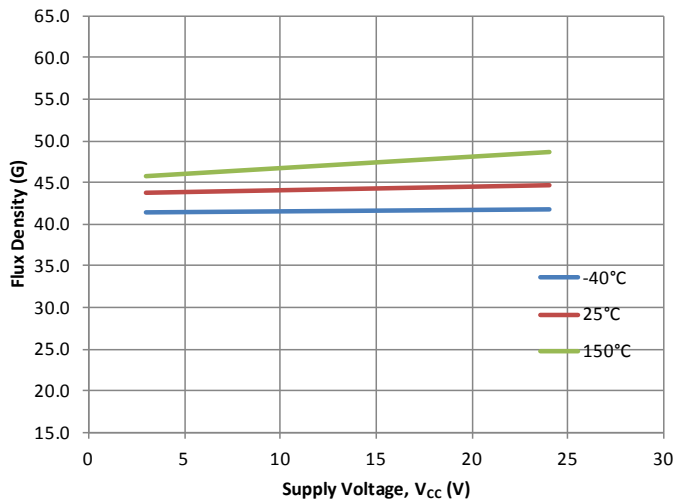
Average B_{HYS} vs. Supply Voltage
