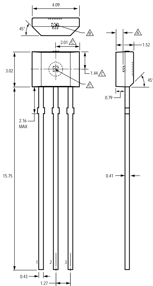
Package UA, Conventional Leadframe
