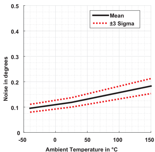
Figure 17: Noise Performance over Temperature (1 \sigma , 300 G)
