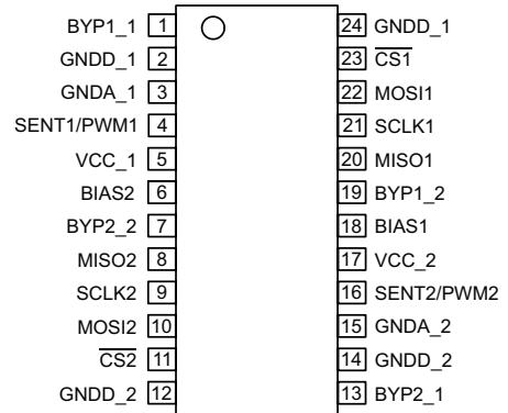
24-Pin TSSOP LE Package Pinouts
