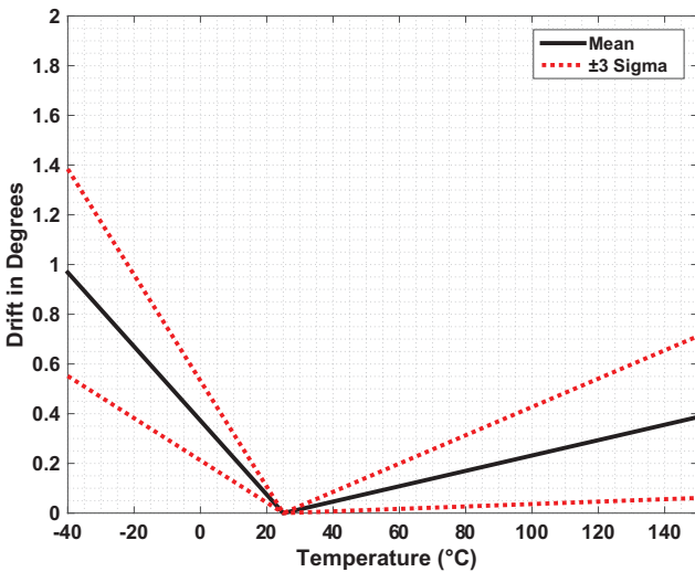
Figure 15: Angle Drift Relative to 25°C (300 G)
