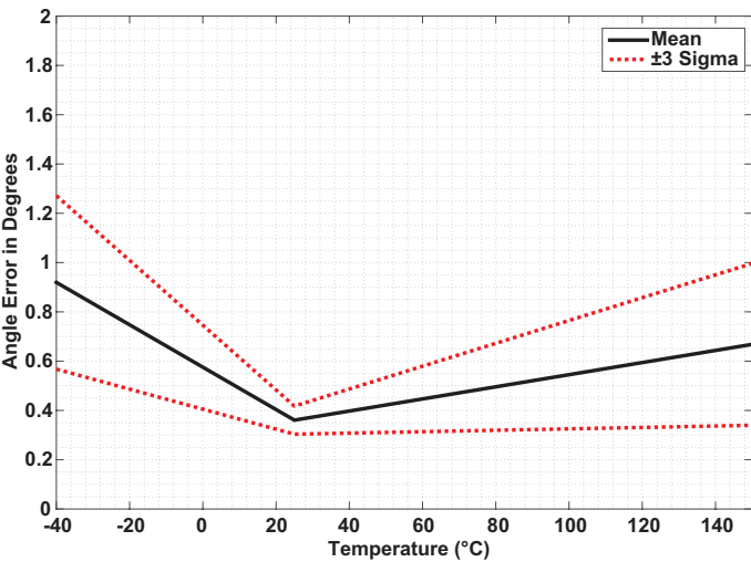
Figure 14: Angle Error over Temperature (300 G)
