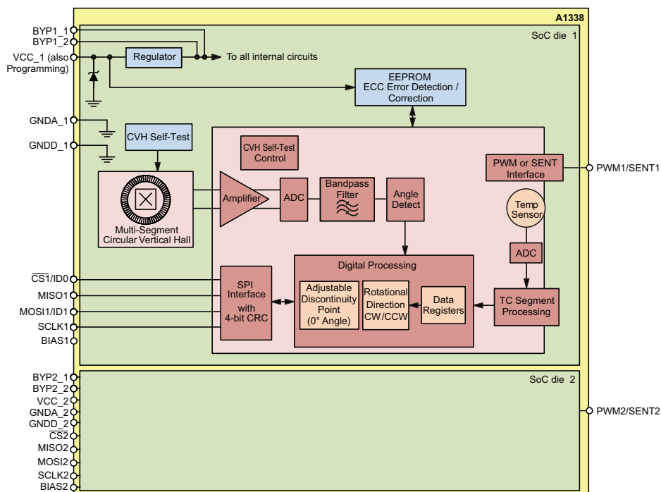
A1338 Magnetic Circuit and IC Diagram
