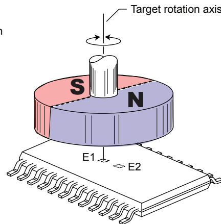
Figure 8: Orientation of Magnet for 0° Relative to Primary Die and 180° Relative to Secondary Die
