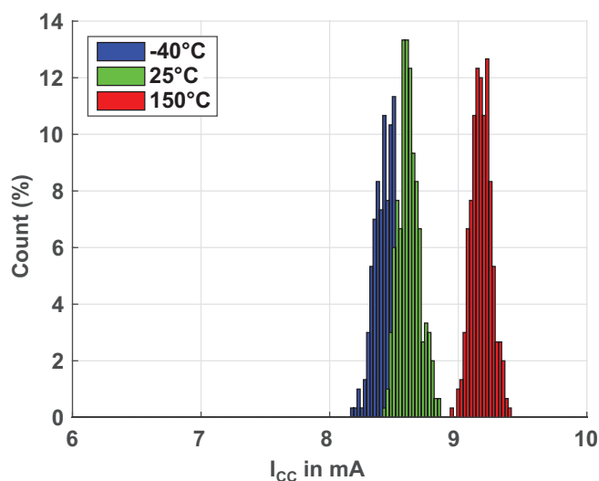
Figure 19: I_{CC} Distribution over Temperature ( I_{CC} per die, V_{CC} = 16 V)
