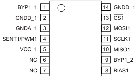
14-Pin TSSOP LE Package Pinouts
