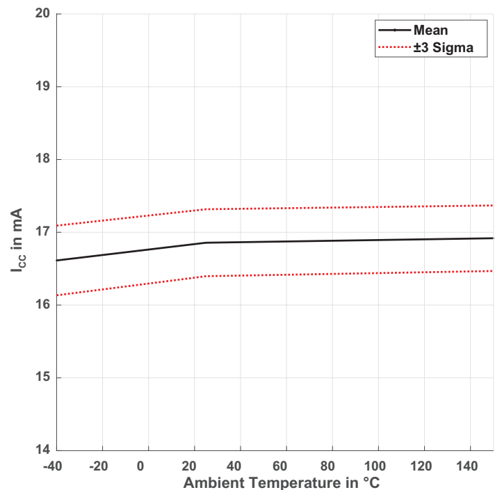
Figure 6: I_{CC} over Temperature ( V_{CC} = 16.0 V)
