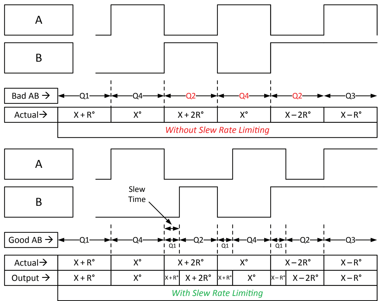
Figure 16: Slew Rate Limiting
