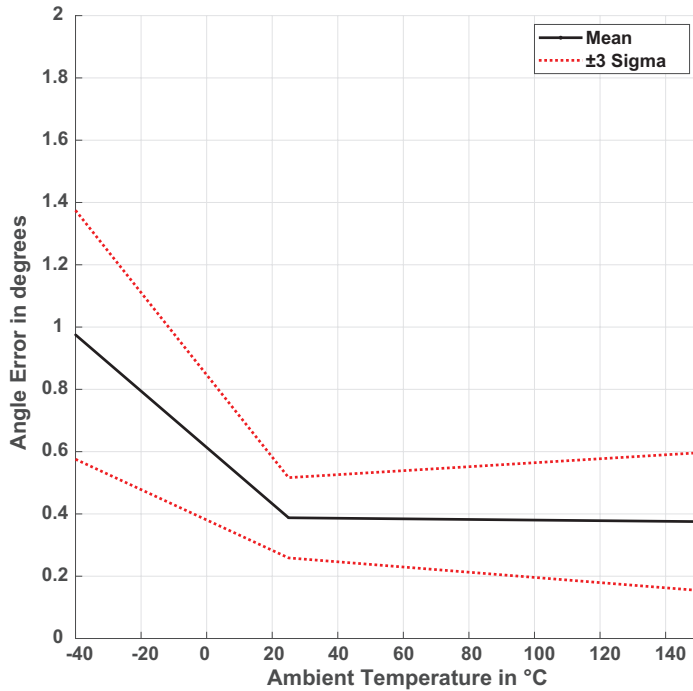
Figure 3: Peak Angle Error over Temperature
