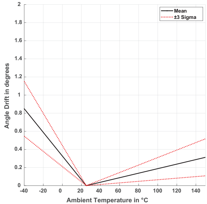
Figure 4: Maximum Absolute Drift from 25°C Reading
