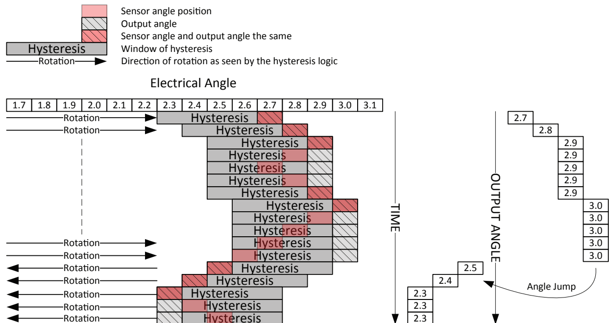
Figure 19: Effect of Hysteresis
