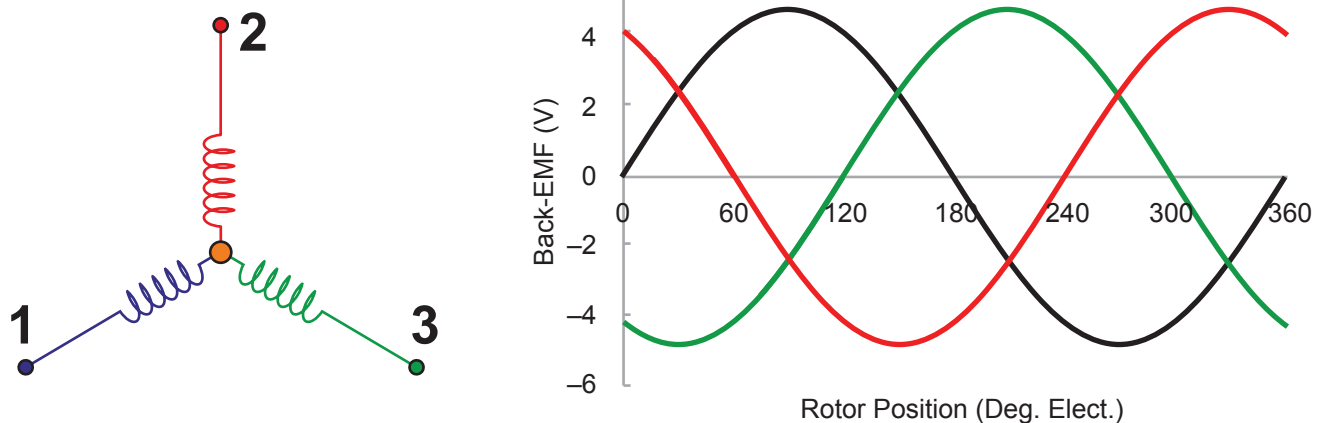
Back-EMF Frequency and Amplitude \propto motor RPM. (Motor BEMF frequency and amplitude are both proportional to motor RPM.)
