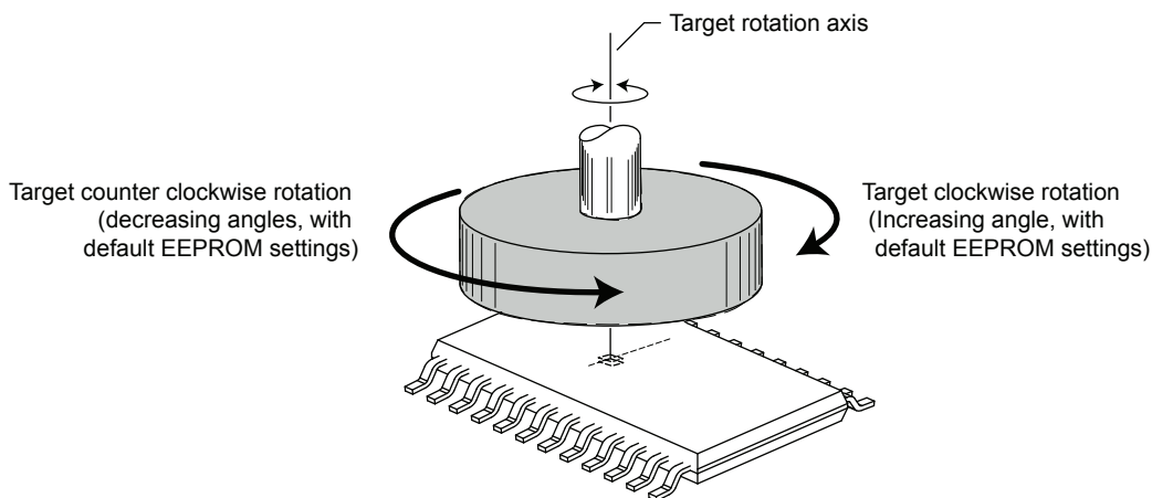
Figure 42: Rotation Direction Definition
