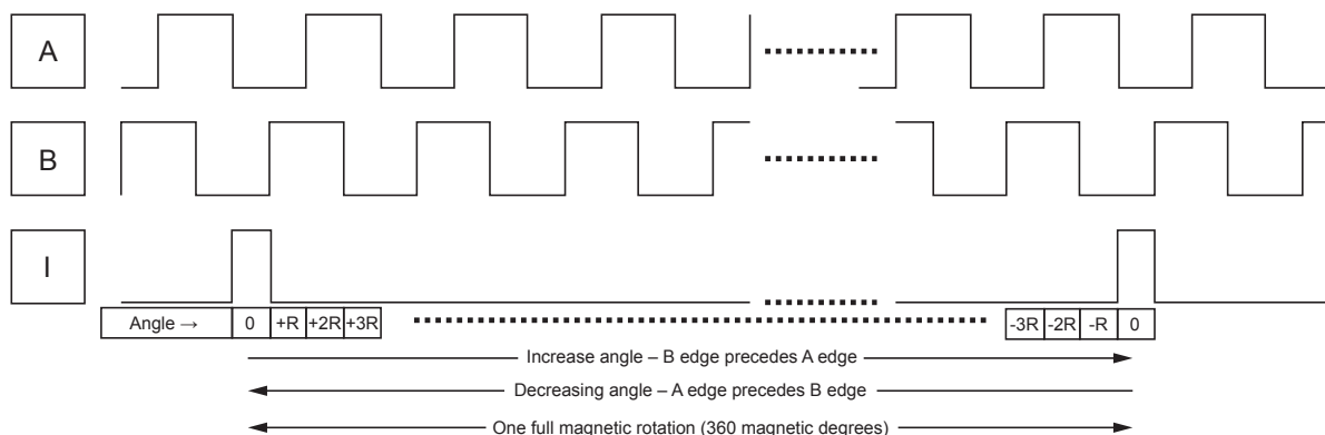
Figure 11: One Full Magnetic Revolution
