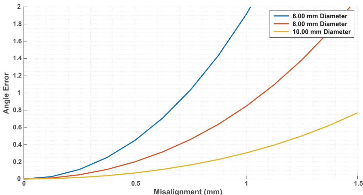
Figure 41: Simulated Error versus Eccentricity for different size magnet diameters, at 2.0 mm air gap
