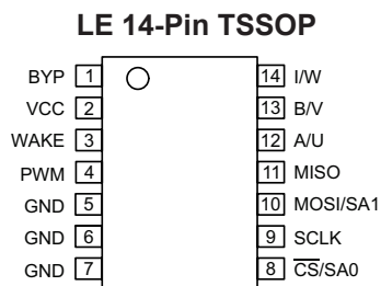
Pinout Diagram
