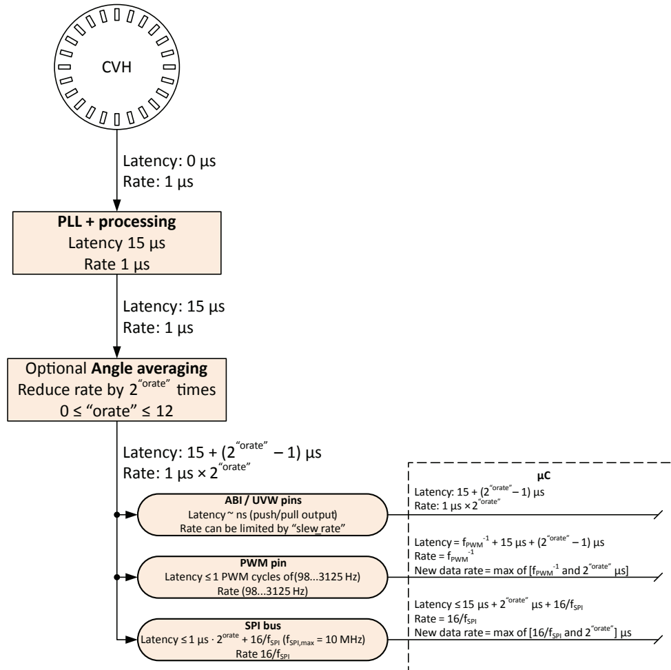
Figure 7: Update Rate and Signal Delay
