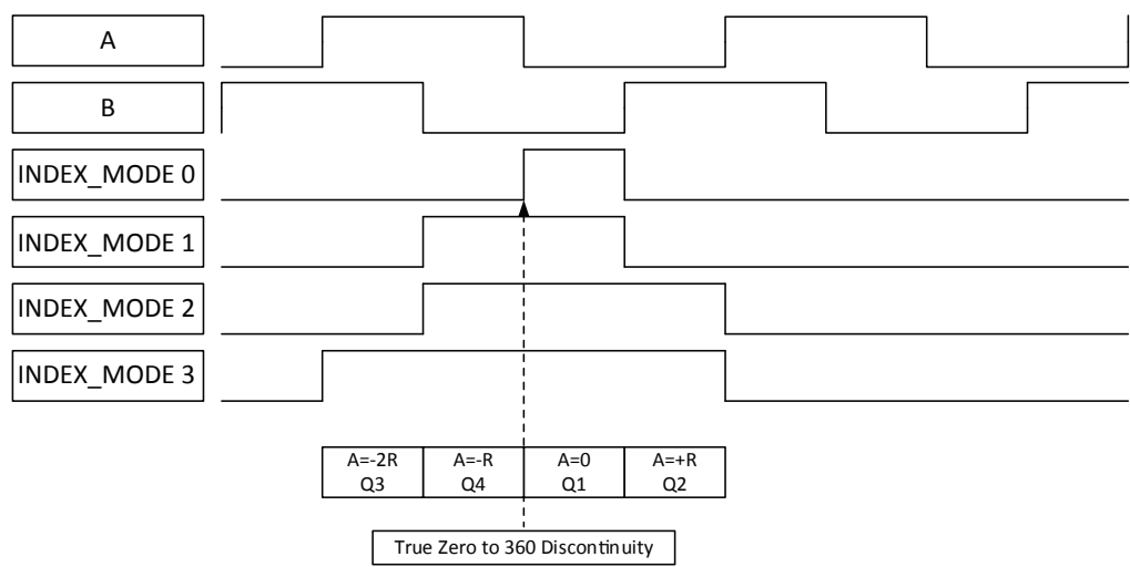
Figure 14: Index Pulse
