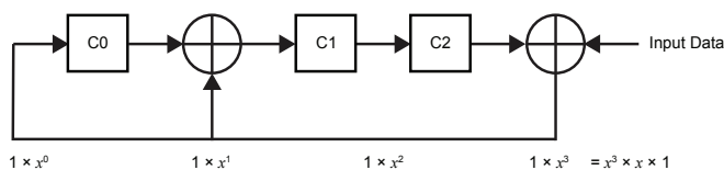
Figure 36: Manchester CRC Calculation
