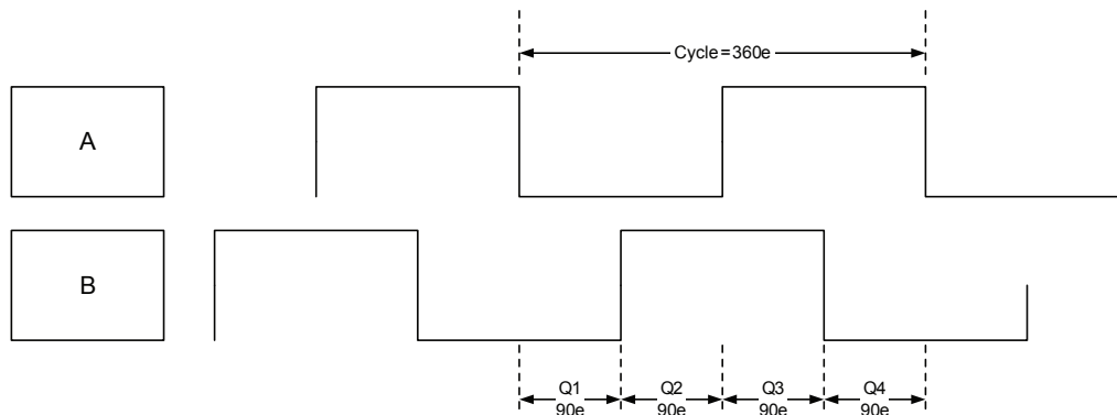
Figure 12: Electrical Cycle
