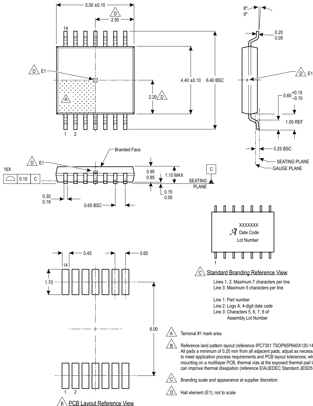
Figure 44: Package LE, 14-Pin TSSOP
