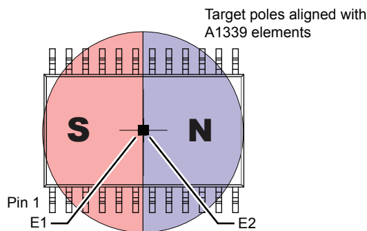
Figure 39: Orientation of Magnet Relative to Primary and Secondary Die
