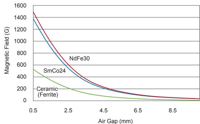
Figure 40: Magnetic Field versus Air Gap for a magnet 6 mm in diameter and 2.5 mm thick.
