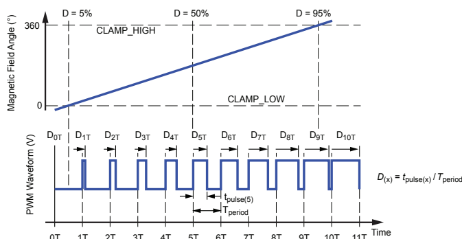
Figure 9: PWM Mode Outputs a Duty-Cycle Proportional To Sensed Angle
