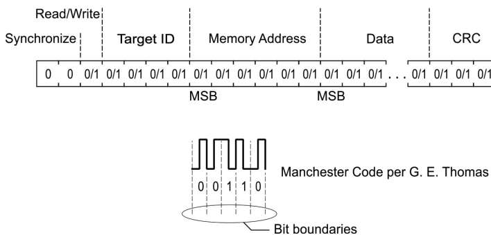
Figure 34: General Format for Serial Interface Commands
