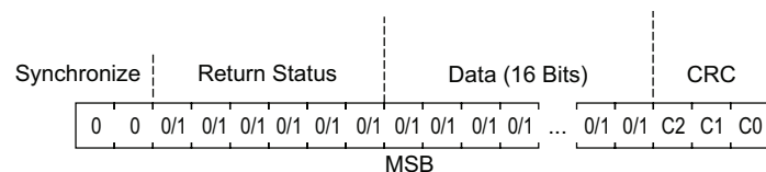
Figure 35: Manchester Read Response
