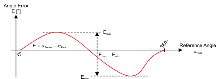
Figure 45: Angle Error Definition
