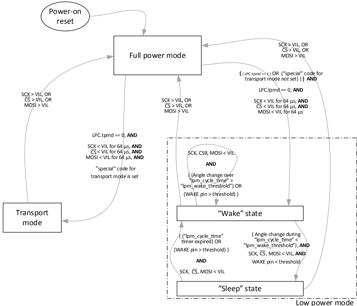
Figure 21: Low Power Mode Flowchart
