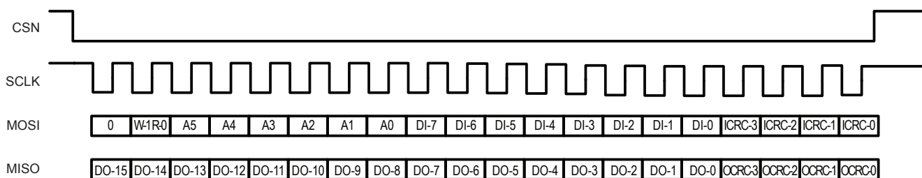
Figure 30: Twenty Bit SPI Transaction
