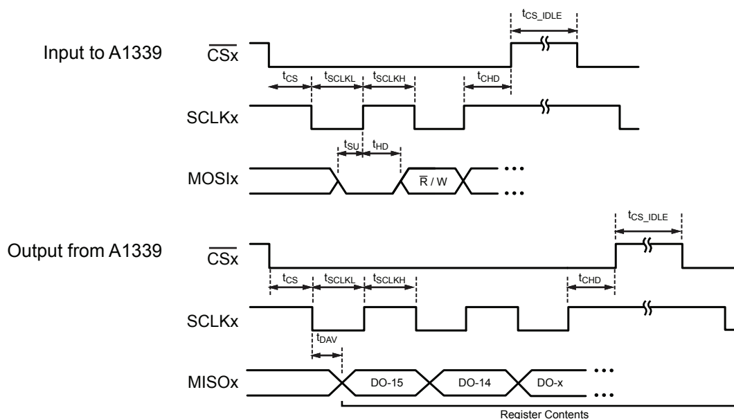
Figure 28: A1339 SPI Interface Timings: (upper) input and (lower) output
