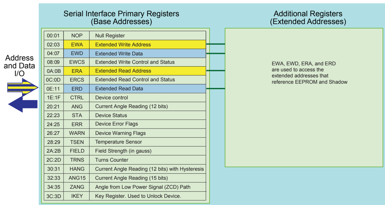
Figure 37: Serial Registers allow access to extended memory (EEPROM and Shadow)
