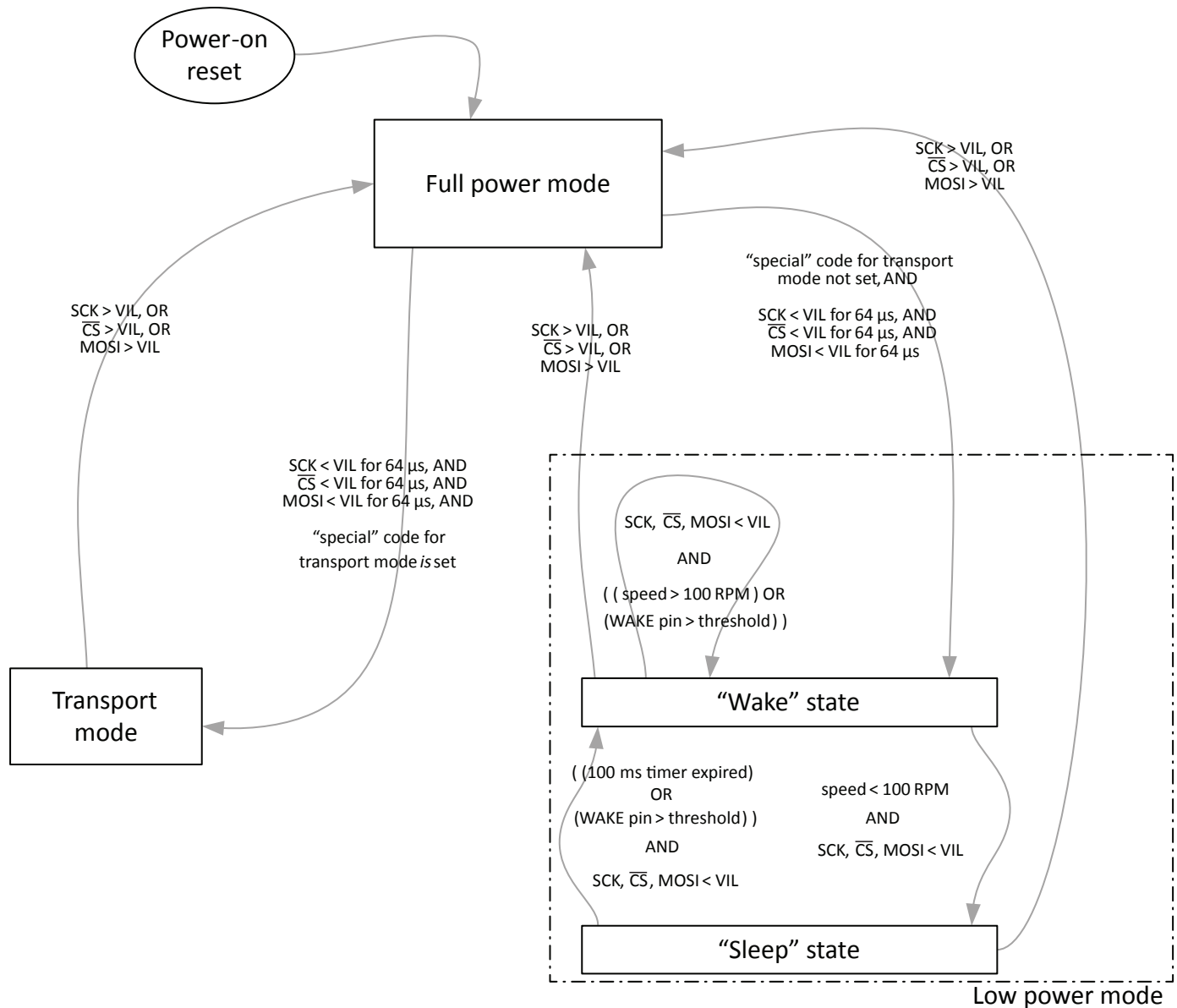
Figure 22: Simplified Low Power Flowchart, Default Settings
