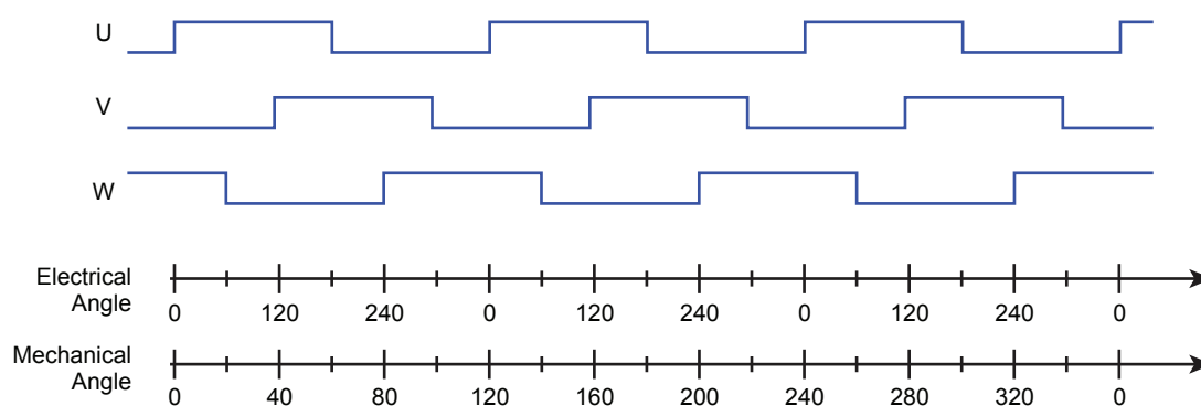
Figure 17: U, V, W Outputs for Three Pole-Pair BLDC Motor
