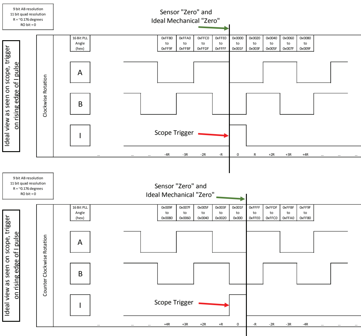
Figure 15: Index Pulse Corresponding to “Zero” Position
