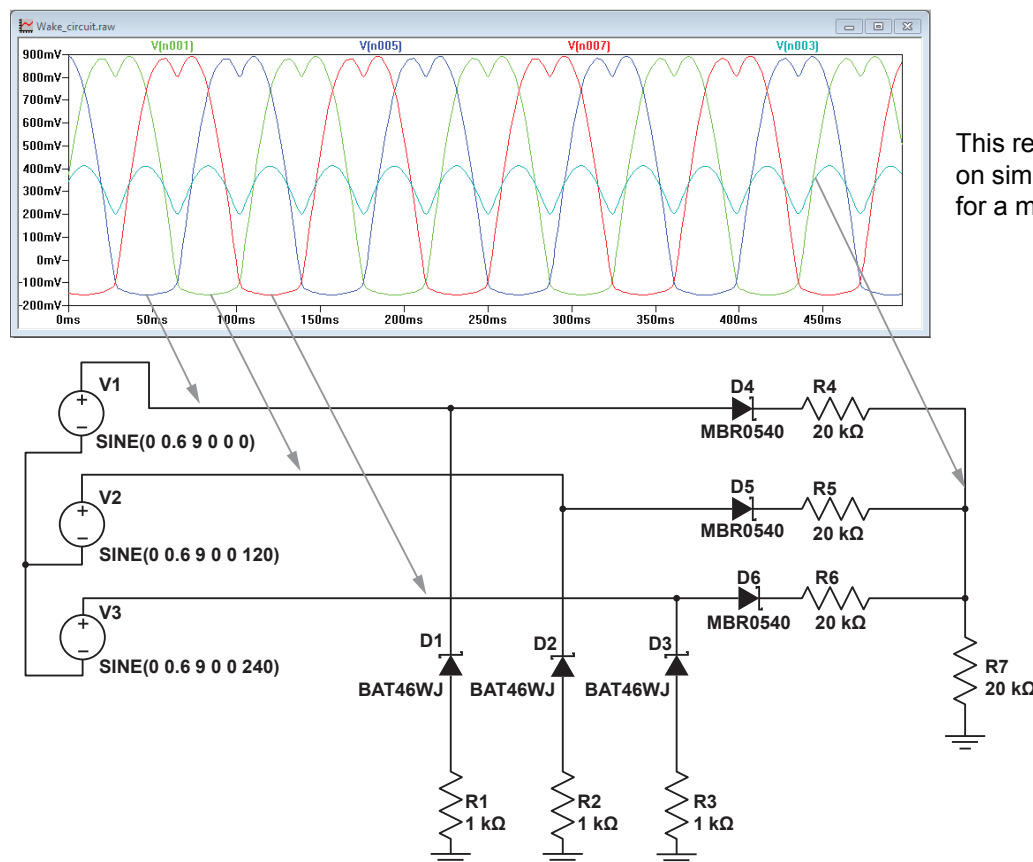
Figure 25: SPICE Simulation Example for Filtered BEMF Signal
