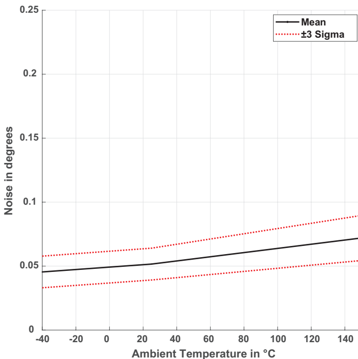
Figure 5: Noise Performance over Temperature (1 Sigma, 300 G)
