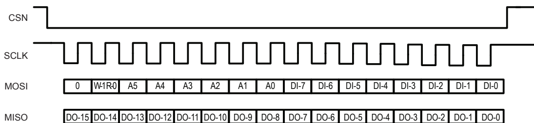
Figure 29: Sixteen Bit SPI Transaction
