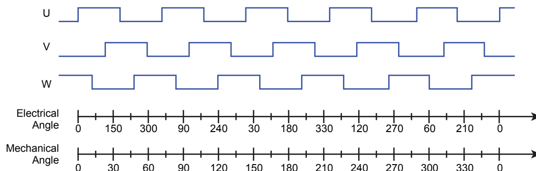
Figure 18: U, V, W Outputs for Five Pole-Pair BLDC Motor
