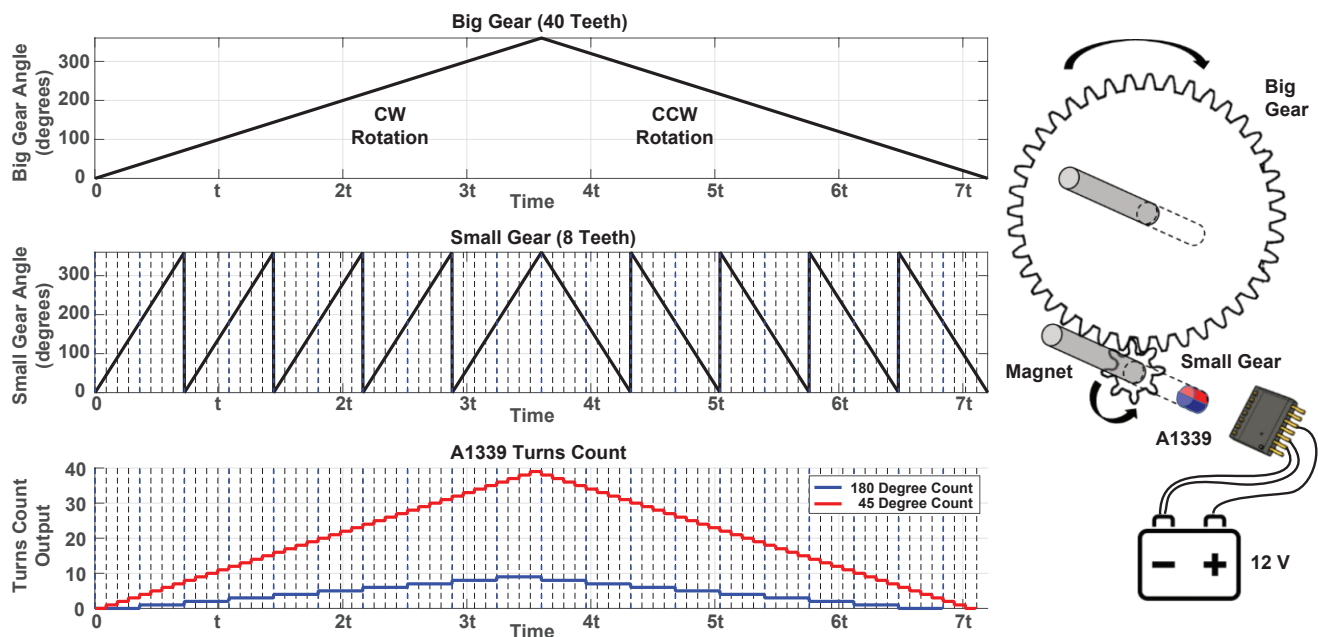
Figure 26: Example of a Turns Counting Application
