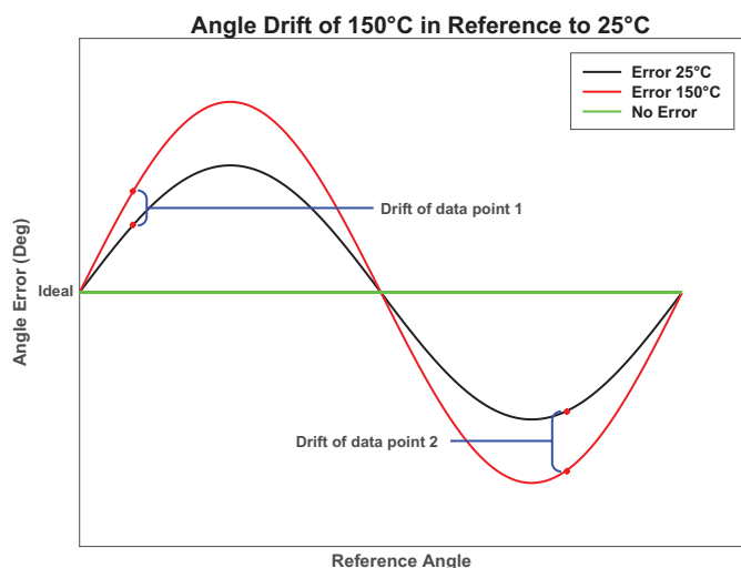
Figure 46: Angle Drift of 150°C in Reference to 25°C [1]
