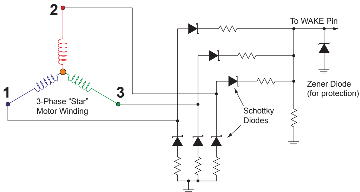
Figure 24: Sample Filtering Circuit
