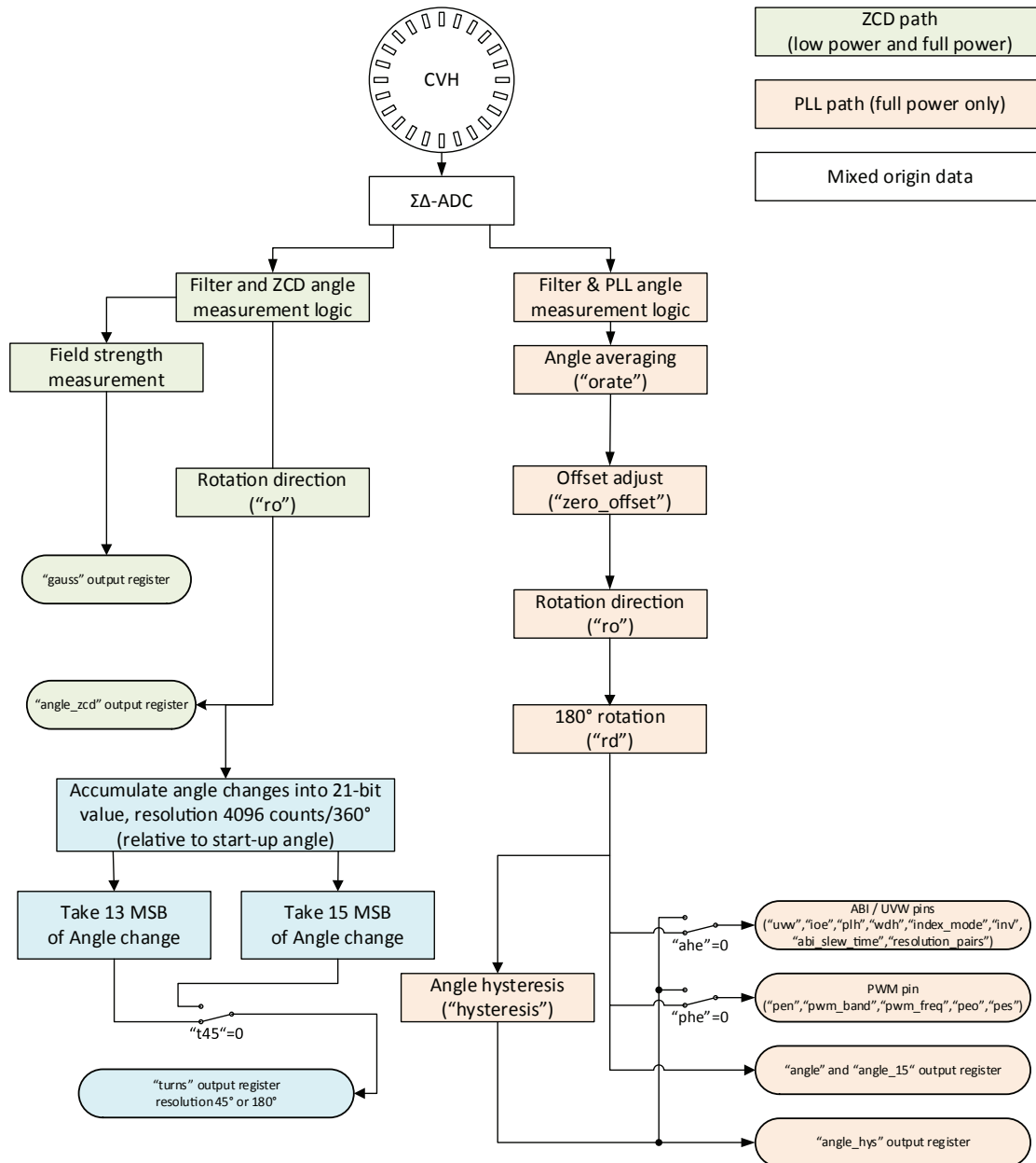
Figure 8: Angle Measurement – Sensor Readout Steps
