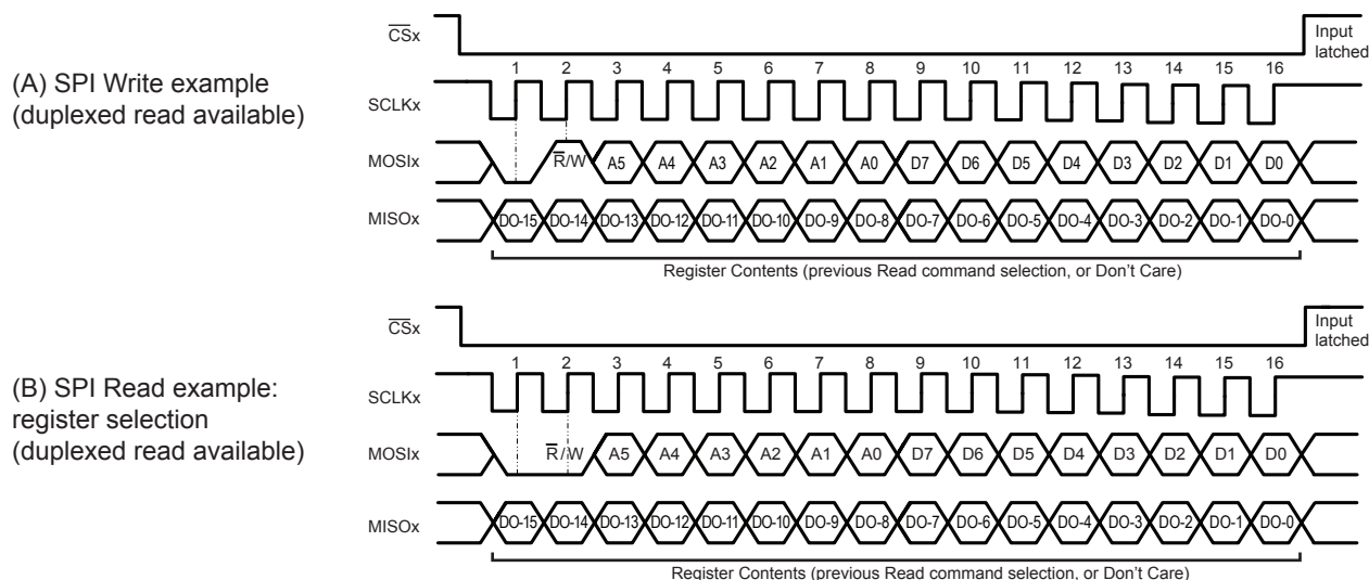
Figure 32: SPI Read and Write Pulse Sequences
