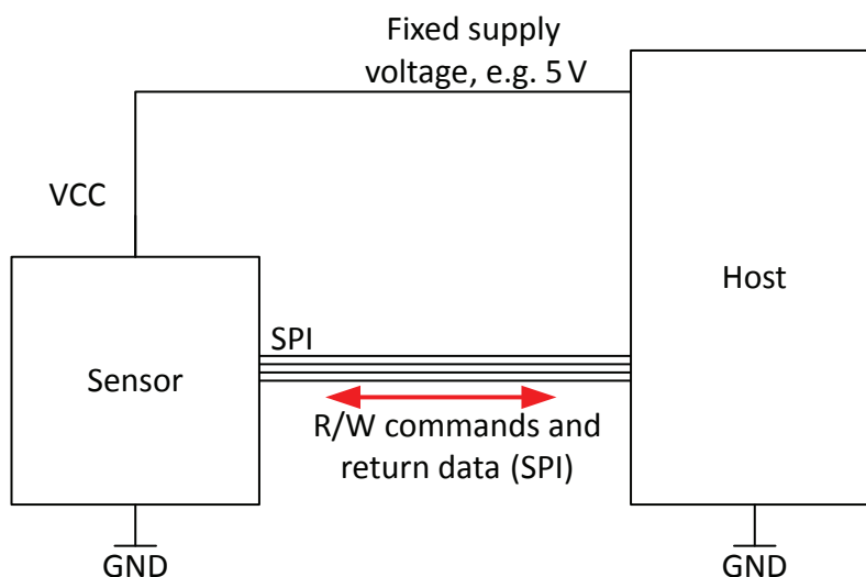
Figure 27: SPI Interface Programming Setup
