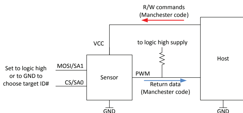
Figure 33: Manchester Interface Programming Setup
