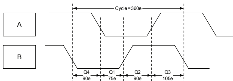
Figure 13: Electrical Cycle
